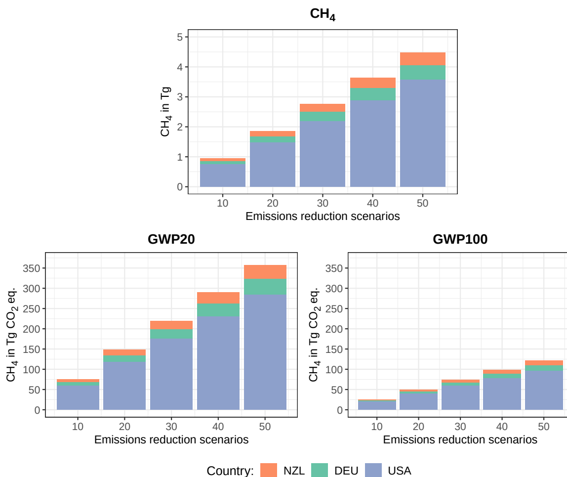
Figure 18: Saved CH 4 through different scenarios (10, 20, 30, 40 and 50%) of a successful shift of rumen microbiome towards less methanogenic microbes. The saved methane is plotted as Tg CH 4 against the these five "Emission reduction scenarios" (CH 4 ). The values for the global warming potential (GWP) for 20 years (79.7) and 100 years (27) are plotted as well in Tg CO 2 eq. (IPCC, 2023a). The saved CH 4 is calculated as an average for the decade 2010-2019 for each country (Germany (DEU), New Zealand (NZL) and United States of America (USA))
