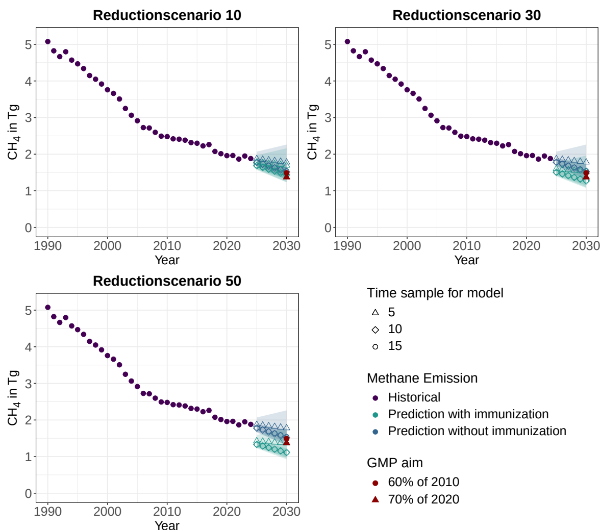
Figure 19: Historical values for total methane emissions in Tg for Germany from 1990 to 2024 and the forecast of methane emissions through 2030. The projection was generated using three different linear models with varying time reference periods (the last 5, 10, or 15 years), which are listed in Table B18 along with the corresponding equation and R^2 . Total emissions were not extrapolated directly. Instead, they were determined using a prediction of total emissions excluding enteric fermentation in cattle, as well as the four indicators (DE, GE, NE x , and herd size), to calculate the missing emissions from cattle production. In addition to predicting total CH 4 emissions without additional mitigation measures (blue), the calculation was also performed for three reduction scenarios (10, 30, and 50% shift in the rumen microbiome) (green). For each linear extrapolation, the confidence interval are displayed as a colored area in the corresponding color (confidence level of 95% was used). The two global methane pledge (GMP) methane emission targets are also shown in red: 60% of 2010 methane emissions as a circle and 70% of 2020 methane emissions as a triangle.
