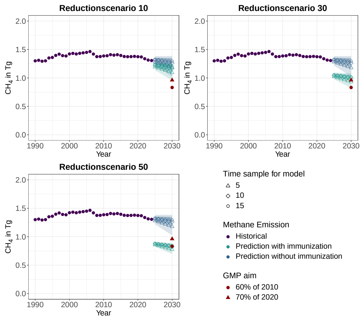
Figure 20: Historical values for total methane emissions in Tg for New Zealand from 1990 to 2024 and the forecast of methane emissions through 2030. The projection was generated using three different linear models with varying time reference periods (the last 5, 10, or 15 years), which are listed in Table B19 along with the corresponding equation and R^2 . Total emissions were not extrapolated directly. Instead, they were determined using a prediction of total emissions excluding enteric fermentation in cattle, as well as the four indicators (DE, GE, NE x , and herd size), to calculate the missing emissions from cattle production. In addition to predicting total CH 4 emissions without additional mitigation measures (blue), the calculation was also performed for three reduction scenarios (10, 30, and 50% shift in the rumen microbiome) (green). For each linear extrapolation, the confidence interval is displayed as a colored area in the corresponding color (confidence level of 95% was used). The two global methane pledge (GMP) methane emission targets are also shown in red: 60% of 2010 methane emissions as a circle and 70% of 2020 methane emissions as a triangle.
