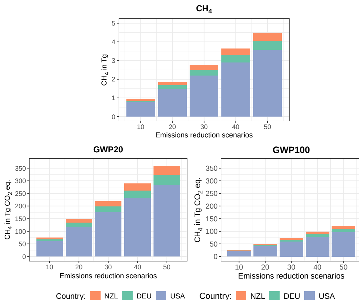
Figure 18: Saved CH 4 through different scenarios (10, 20, 30, 40 and 50%) of a successful shift of rumen microbiome towards less methanogenic microbes. The saved methane is plotted as Tg CH 4 against the these five "Emission reduction scenarios" (CH 4 ). The values for the global warming potential (GWP) for 20 years (79.7) and 100 years (27) are plotted as well in Tg CO 2 eq. (IPCC, 2023a). The saved CH 4 is calculated as an average for the decade 2010-2019 for each country (Germany (DEU), New Zealand (NZL) and United States of America (USA))
