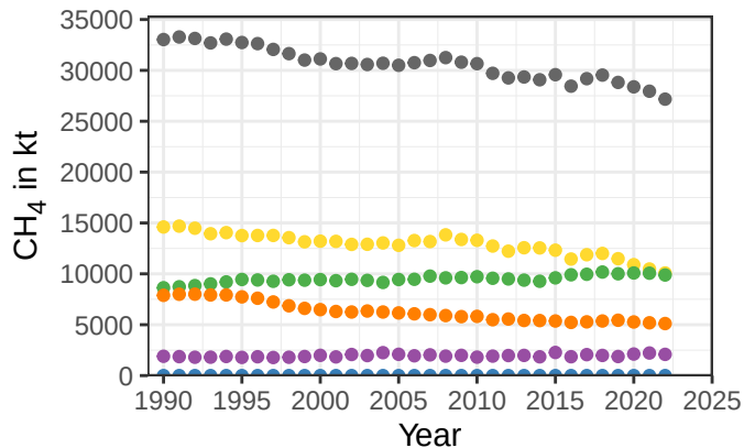
Emissionsectors – USA
