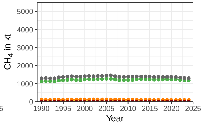
Emissionsectors – NZL
