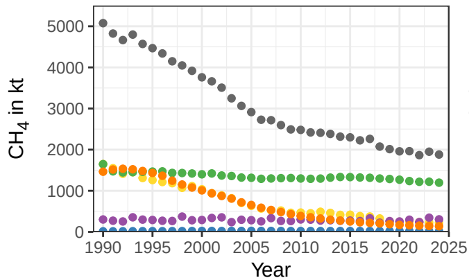
Emissionsectors – USA
