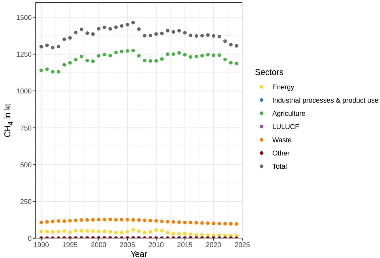
Emissionsectors – NZL
