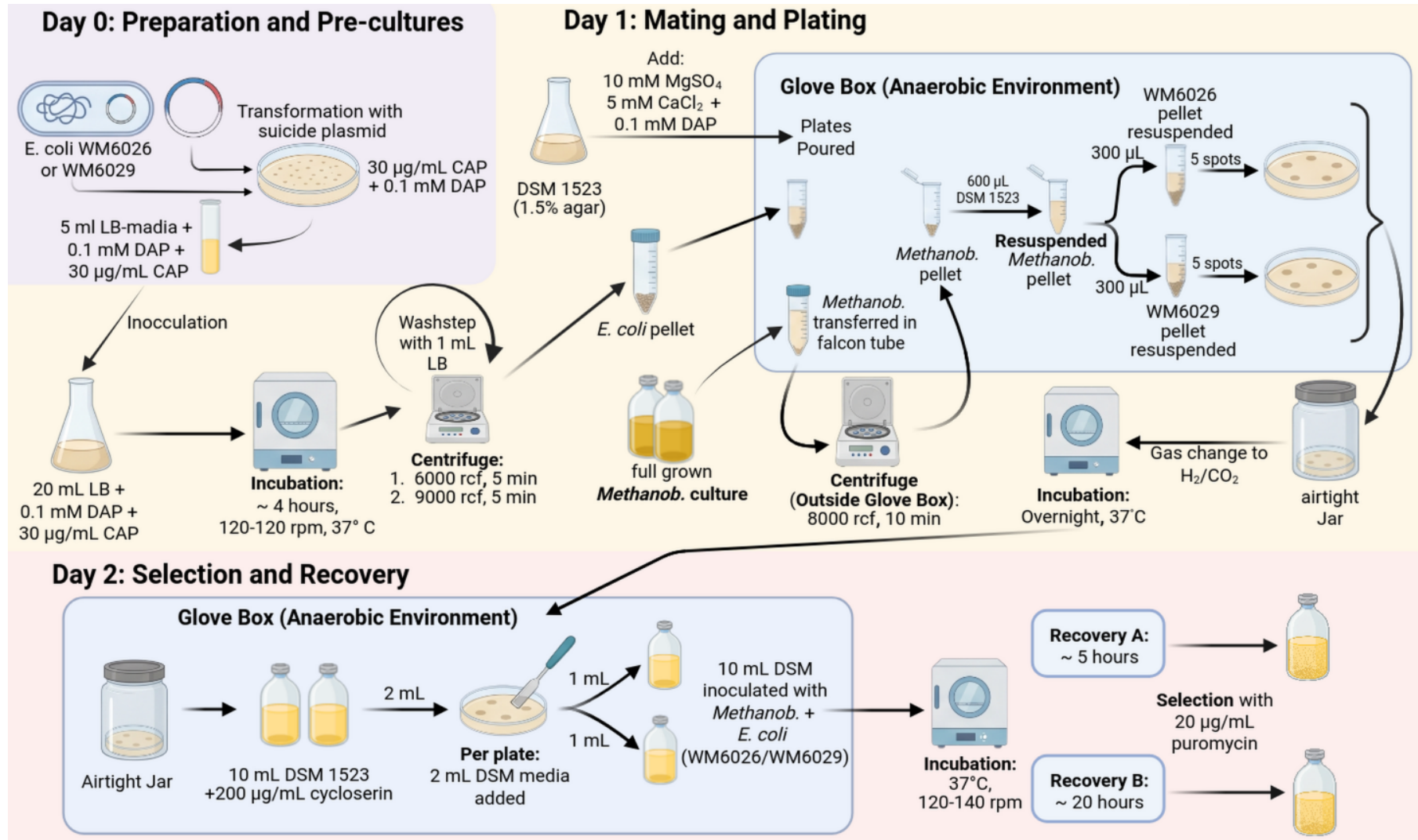
Figure 4: Methodological approach to transform a Methanobrevibacter ( Methanob. ) species via interdomain conjugation using two diaminopimelic acid (DAP) auxotrophic E. coli strains, WM6026 and WM6029. Suicide plasmids corresponding to the targeted Methanob. species were used, containing chloramphenicol (CAP) as a selection marker for E. coli and puromycin as a selection marker for the transformed Methanob. Two recovery periods were tested: Recovery A (approx. 5 h) and Recovery B (approx. 20 h).
