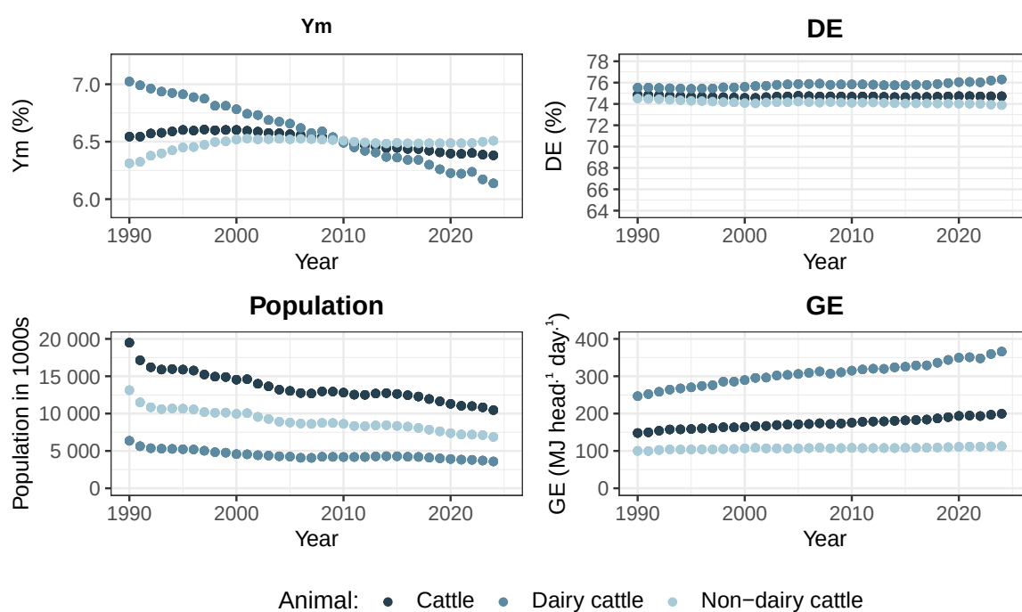
Figure A4: Time series of methane conversion factor (Ym), population-size, digestibility of food (DE) and gross energy intake (GE) of cattle and its subcategories dairy and non-dairy for DEU. The data for dairy and non-dairy cattle is from the published CRT. The values for cattle is calculated as weighted mean of its subcategories, where the population-size is used as weight.
