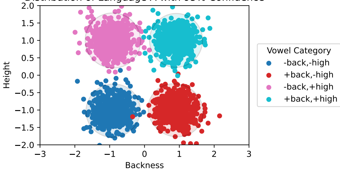
Distribution of Language A with 95% Confidence
