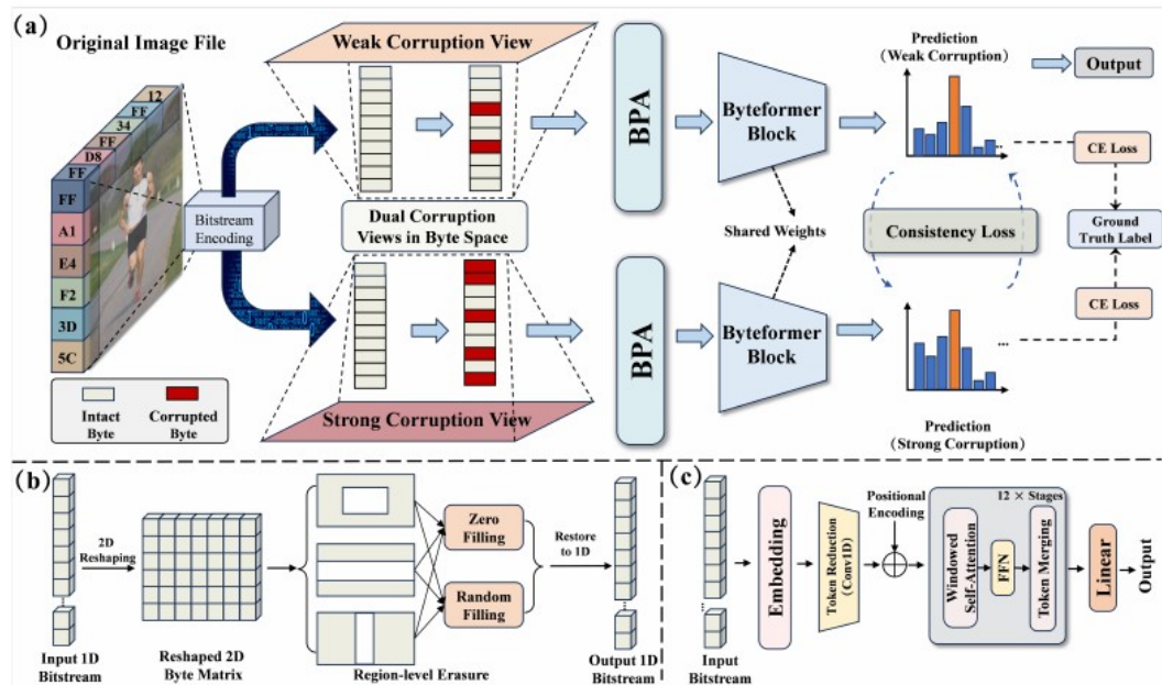
Figure 2: Overview of the proposed ByteAction framework. (a) ByteAction constructs dual corruption views in byte space from the input image bitstream, including weakly and strongly corrupted views. The two views are augmented by Bitstream Pattern Augmentation (BPA), encoded by a shared-weight ByteFormer backbone, and optimized with both cross-entropy
