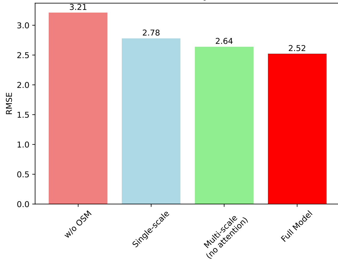
Ablation Study: RMSE
