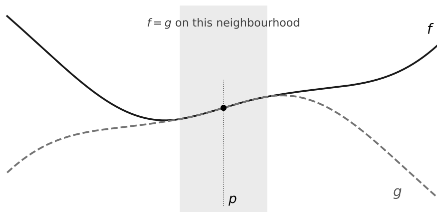
Figure 3.2: Two functions with the same germ at p : they agree on a neighbourhood of p , and may do as they please elsewhere.
