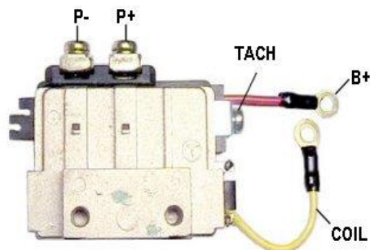
IGN MODULE NM746
