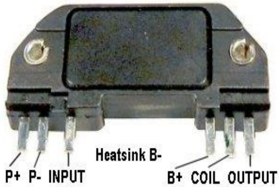
IGN MODULE TP800D MODULE OPEL KADET MONZA
