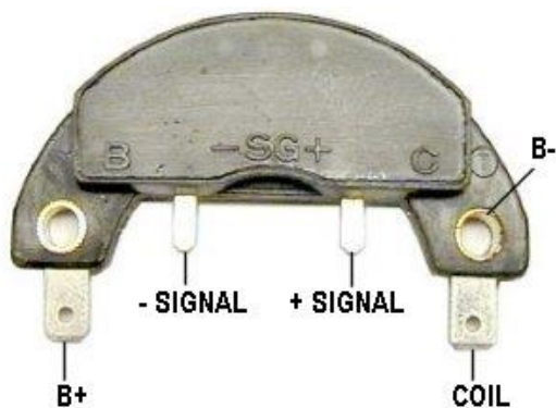
IGN MODULE TP1000M MAGNETIC TRIGGER MAZDA 4P
