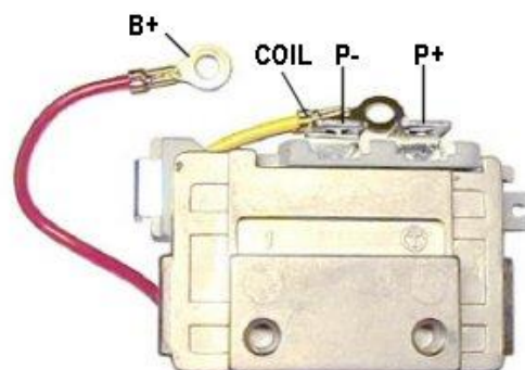
IGN MODULE TP189 IGN MOD TOYOTA COROLLA 1.3/1.6
