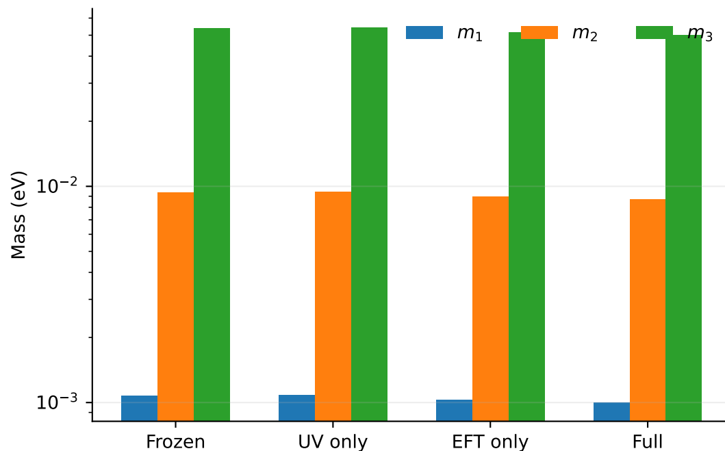
Leptonic mixing
