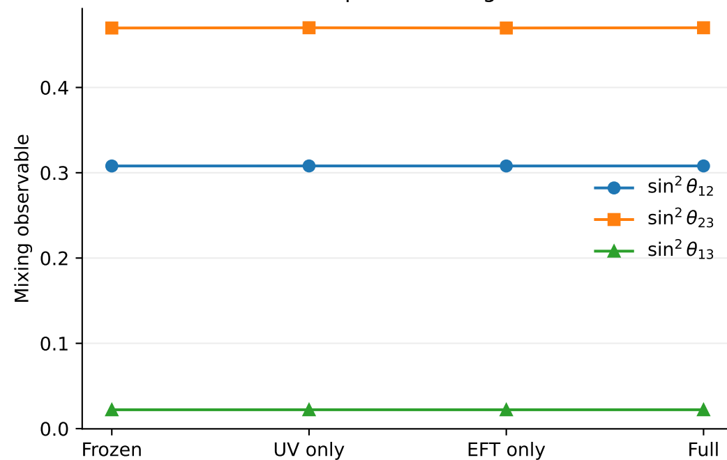
Leptonic mixing
