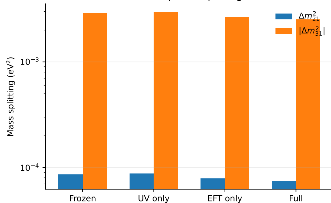
Mass-squared splittings
