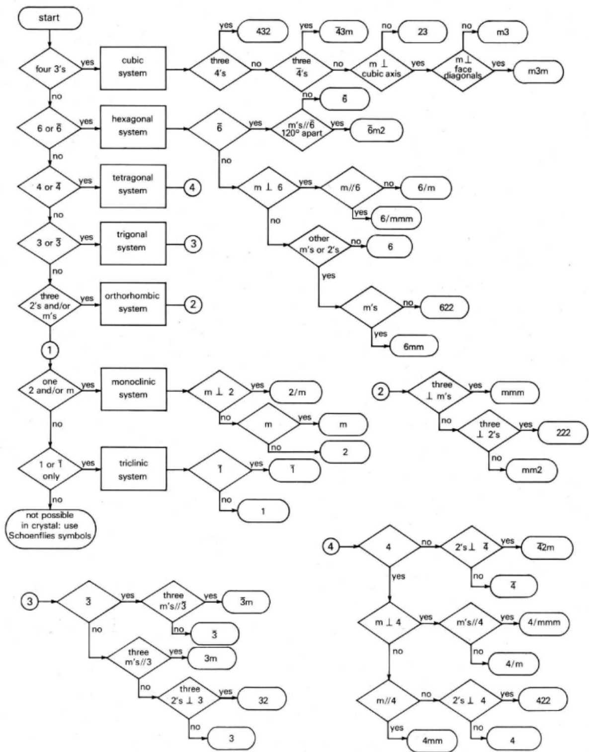
Hermann-Mauguin symmetry notation flow chart. (// reads "parallel to.")
