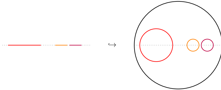
Figure 2: example of a configuration of E_1 being embedded in E_2 along the horizontal line
