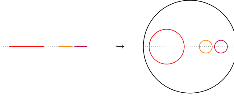
Figure 2: example of a configuration of E_1 being embedded in E_2 along the horizontal line
