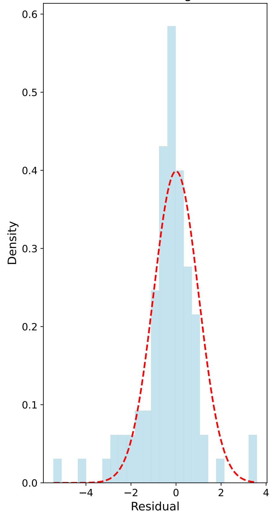
Residual histogram
