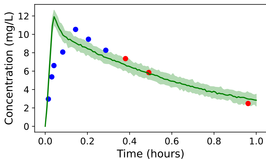
Test Individual 2
