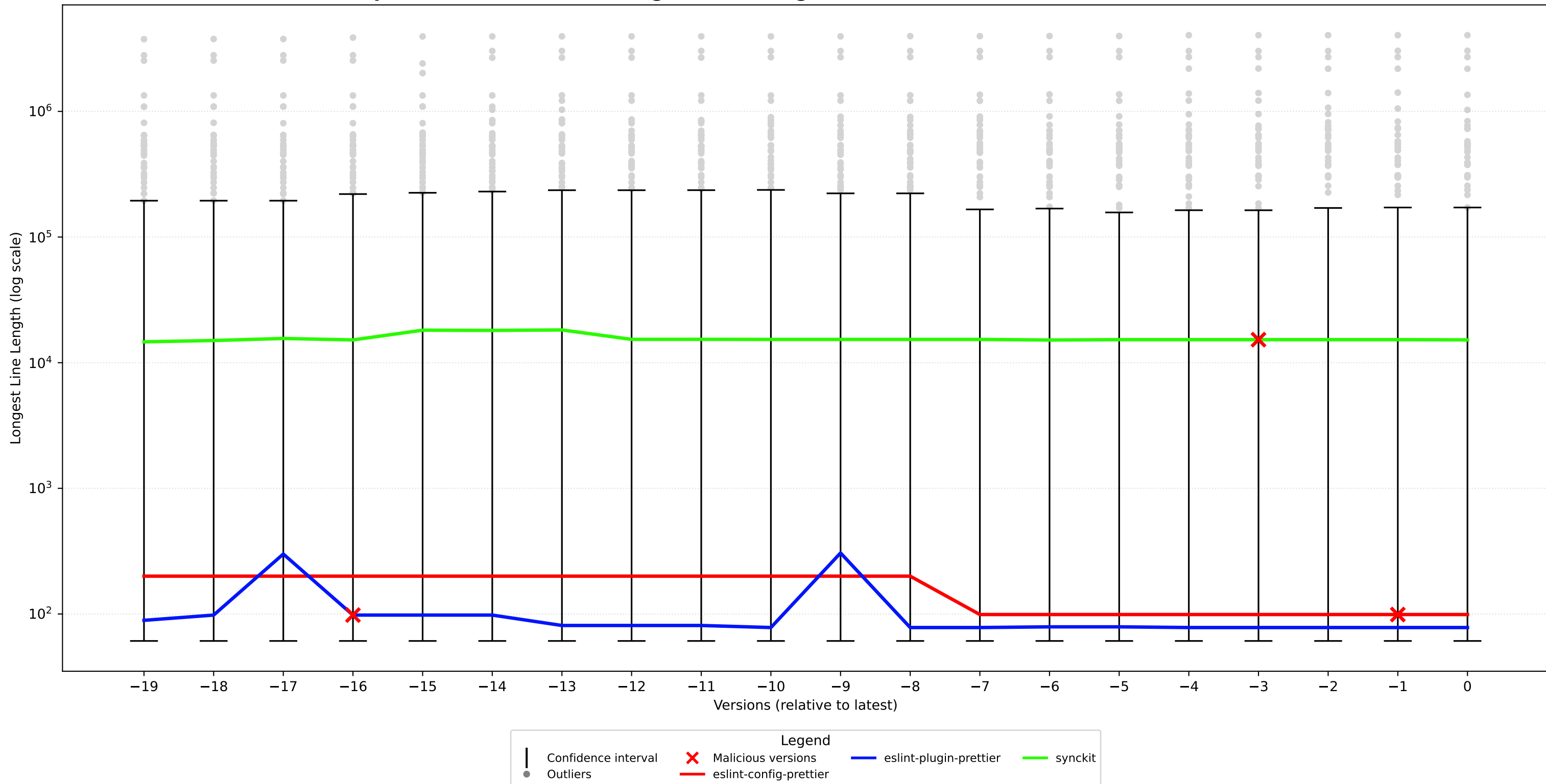
Comparison with Malware Longest Line Length Metric - Attack A: Malicious Windows DLL
