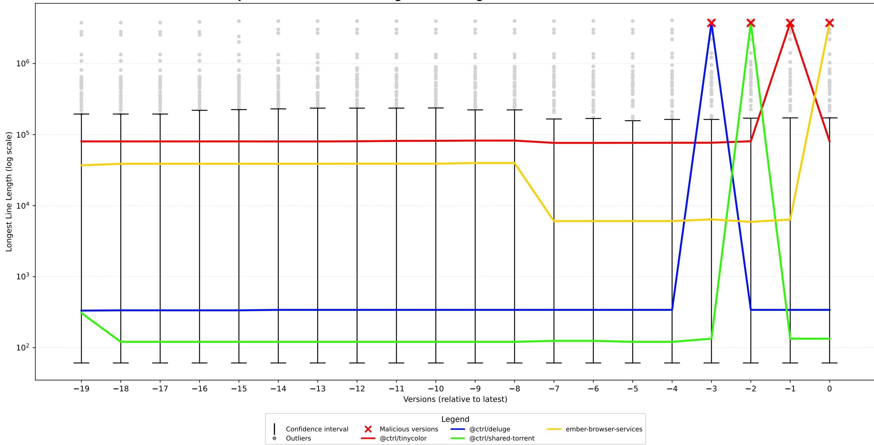
Comparison with Malware Longest Line Length Metric - Attack C: Shai-Hulud 1.0
