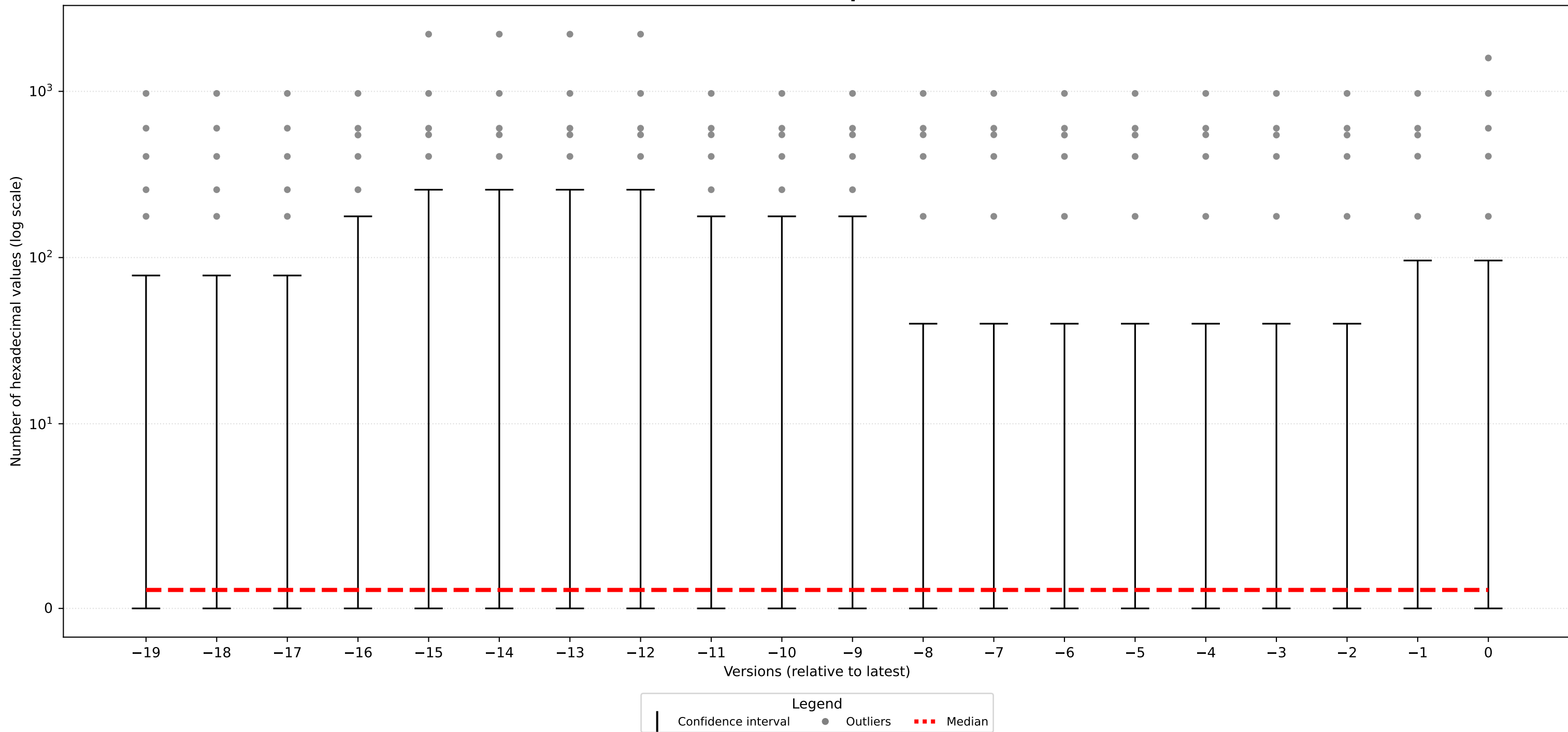
Goodware dataset Trend for the Unique Hexadecimal values Metric
