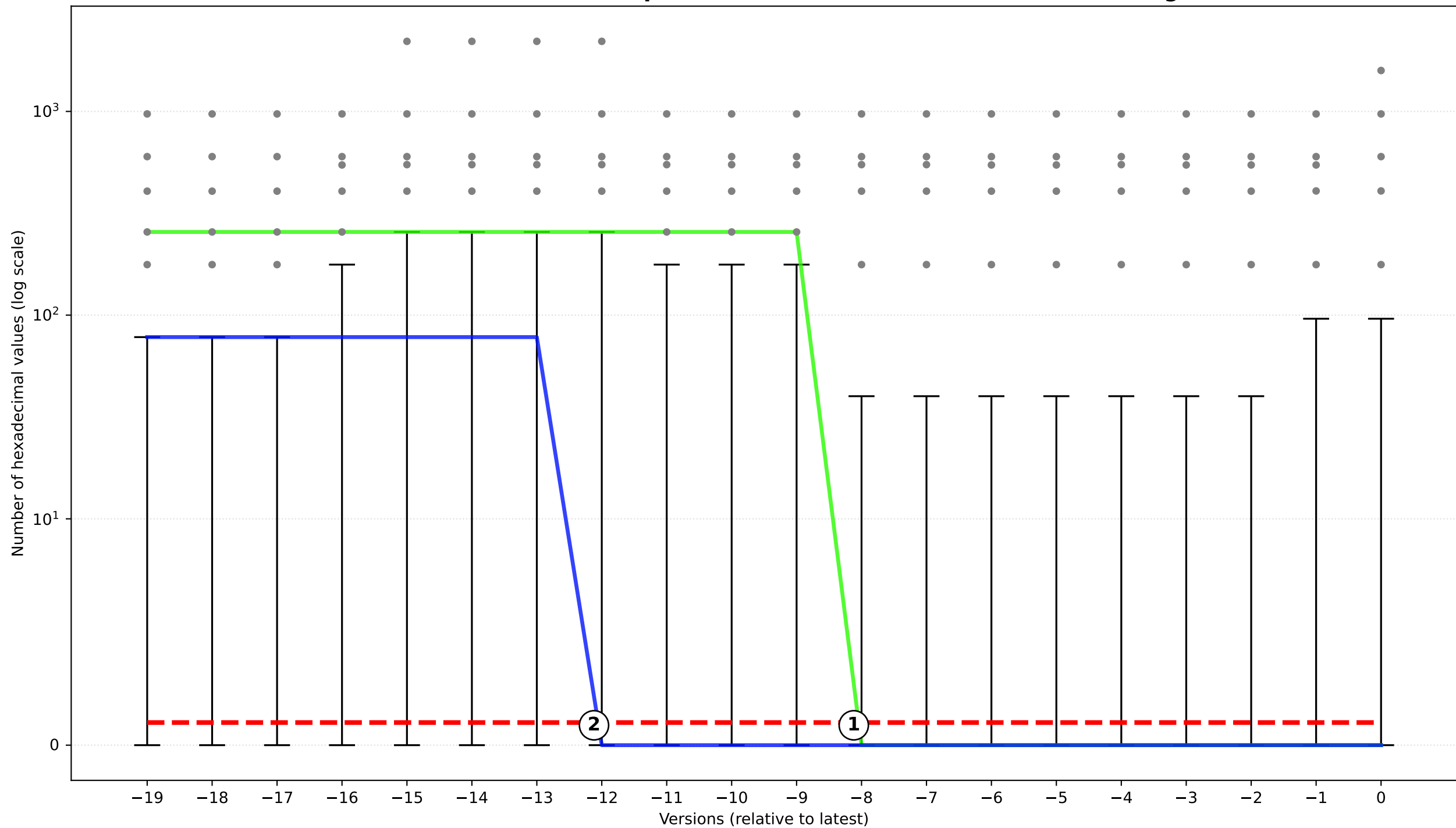
Goodware dataset for the Unique Hexadecimal values Metric - Decreasing Trend
