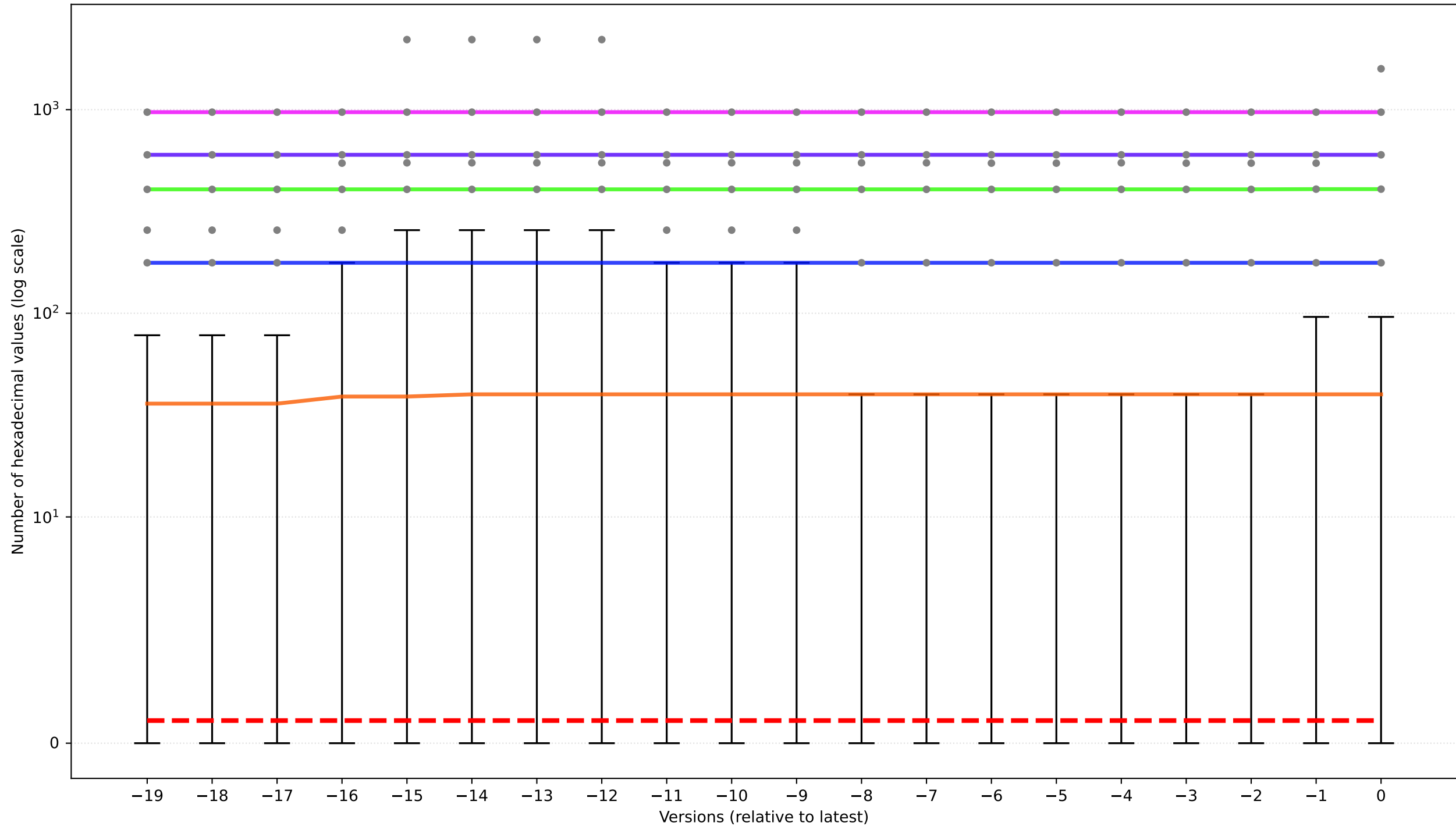
Goodware dataset for the Unique Hexadecimal values Metric - Stable Trend
