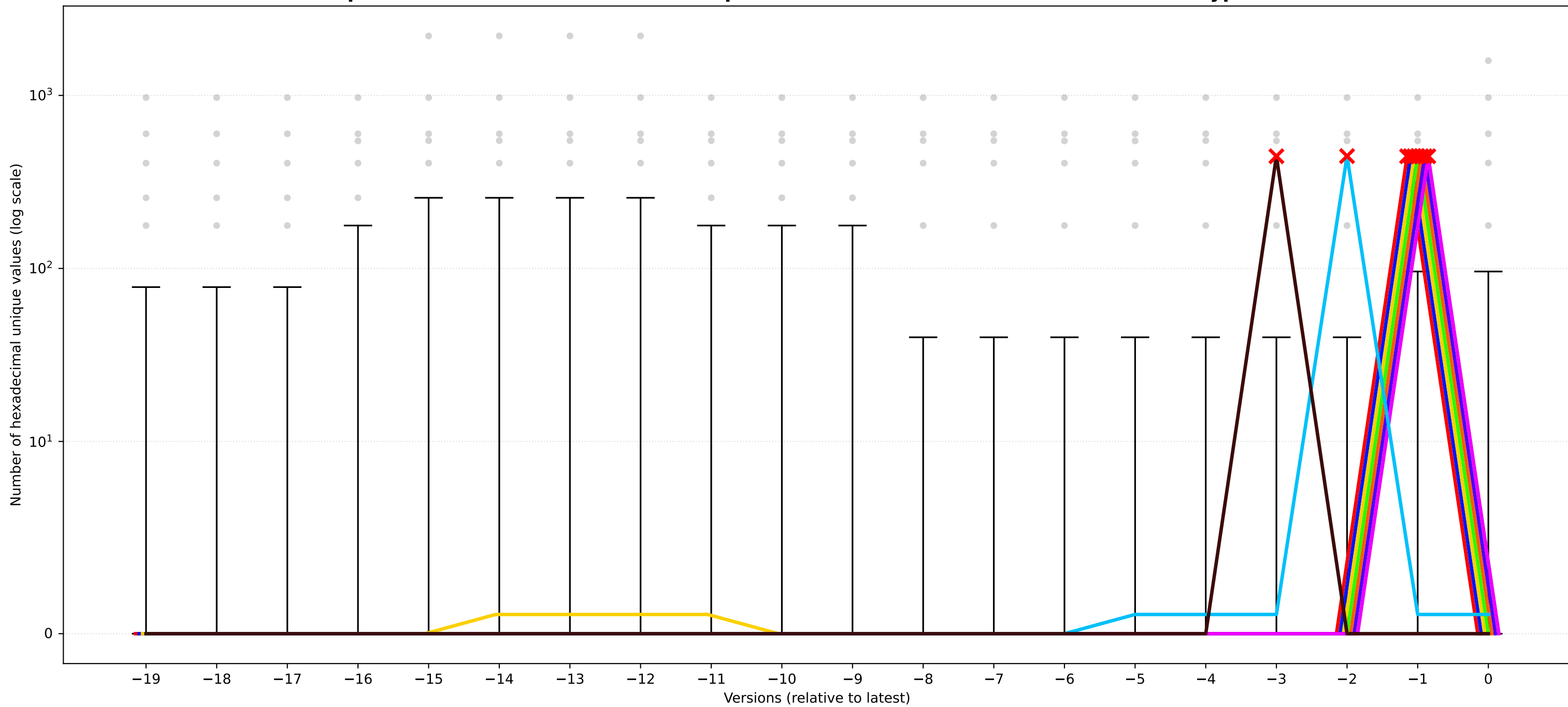
Comparison with Malware Dataset Unique Hexadecimal values Metric - Attack B: Crypto attack
