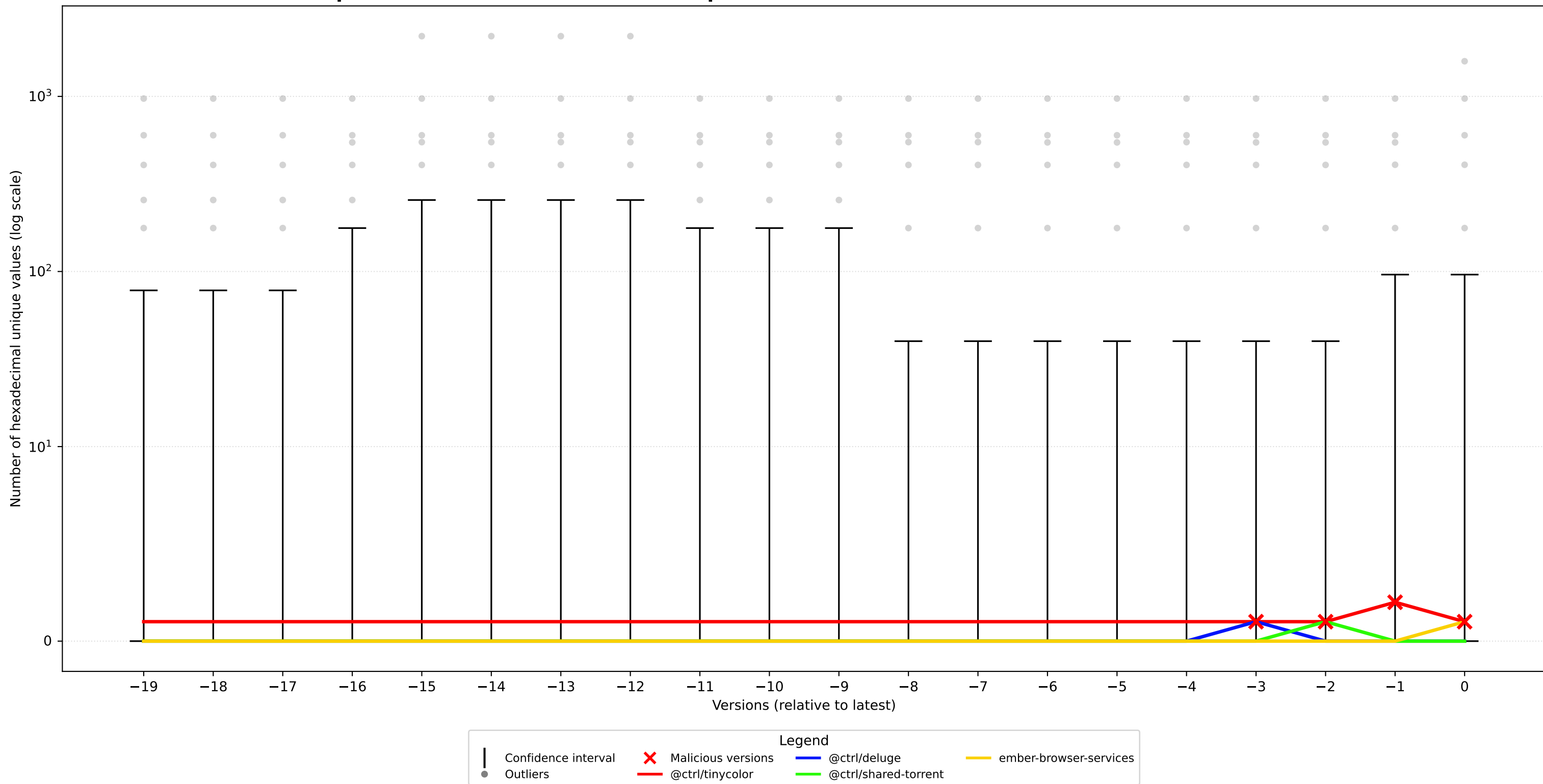
Comparison with Malware Dataset Unique Hexadecimal values Metric - Attack C: Shai-Hulud 1.0
