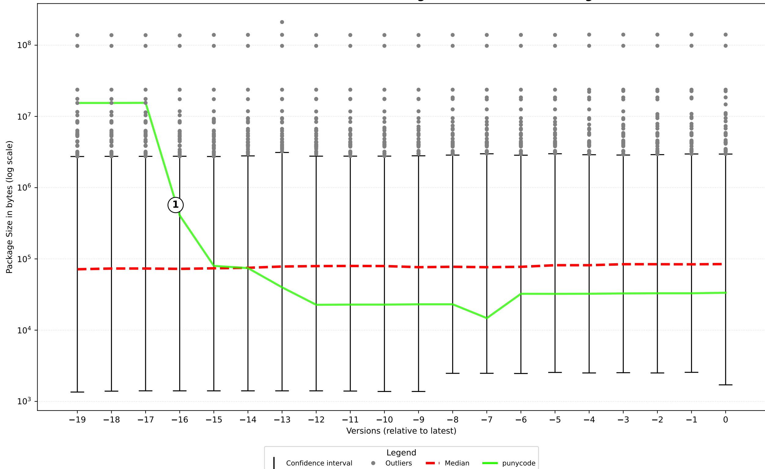
Goodware dataset Trend for the Package Size Metric - Decreasing Trend
