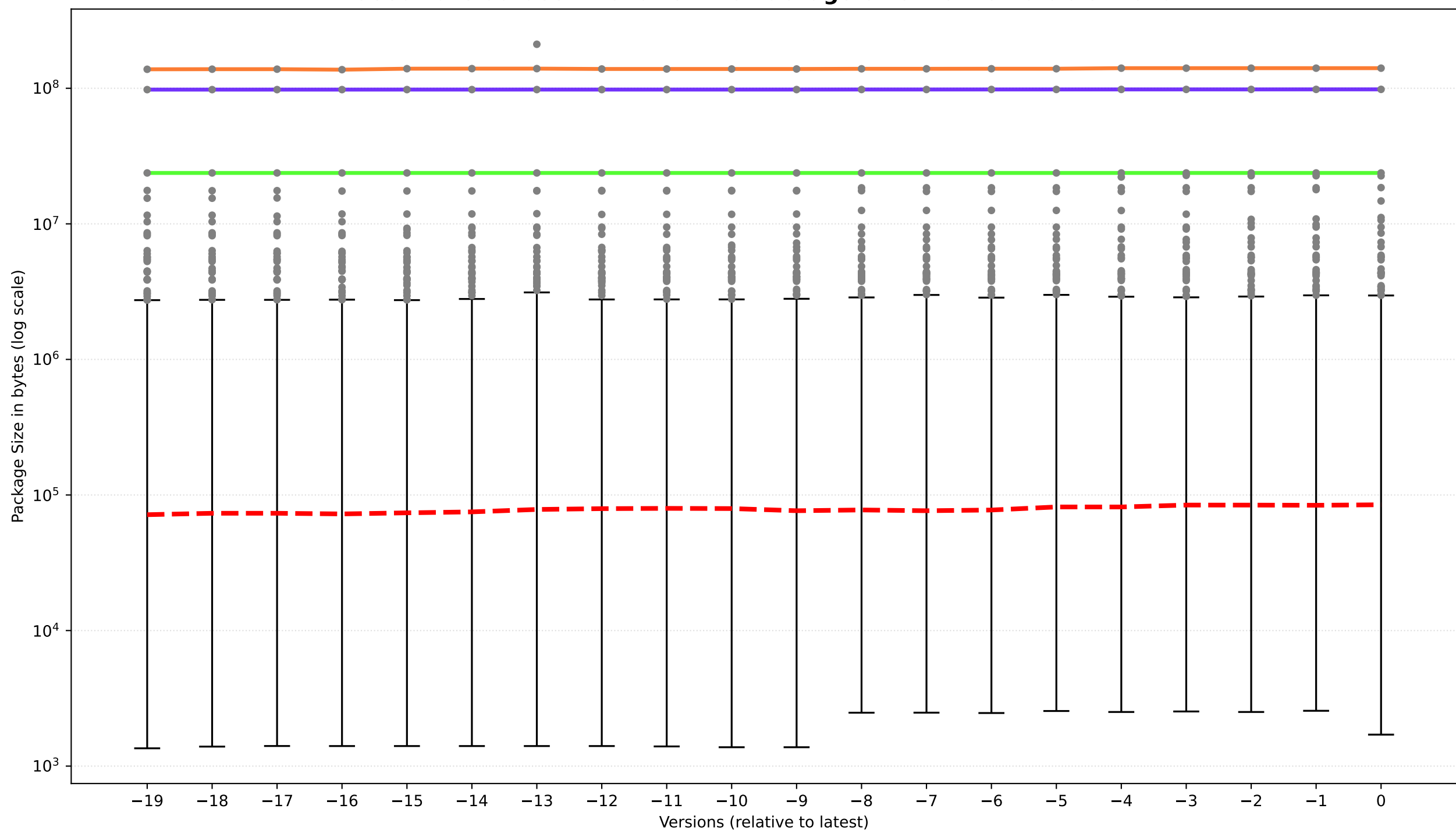
Goodware dataset Trend for the Package Size Metric - Stable Trend
