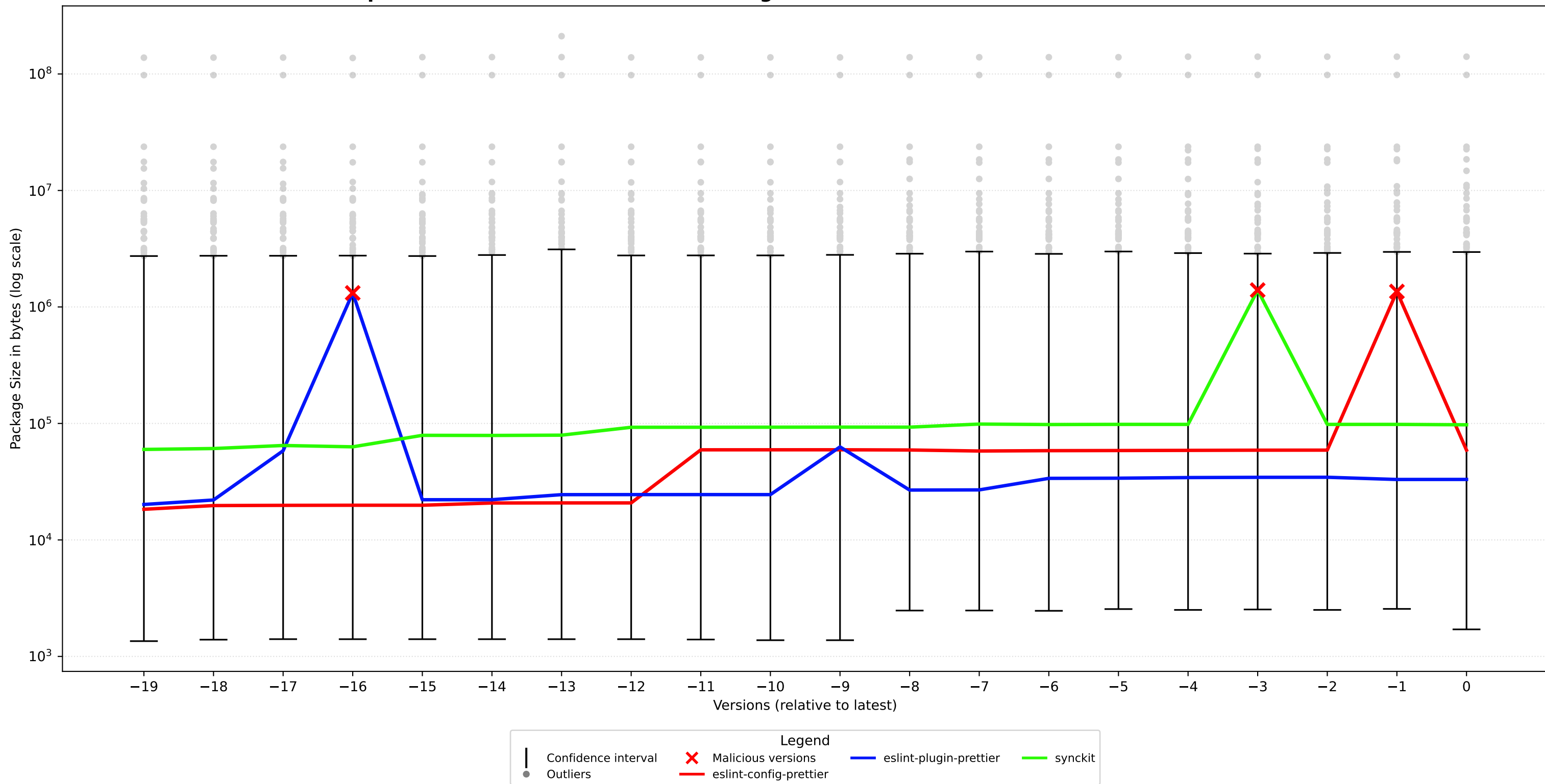
Comparison with Malware Dataset Package Size Metric - Attack A: Malicious Windows DLL
