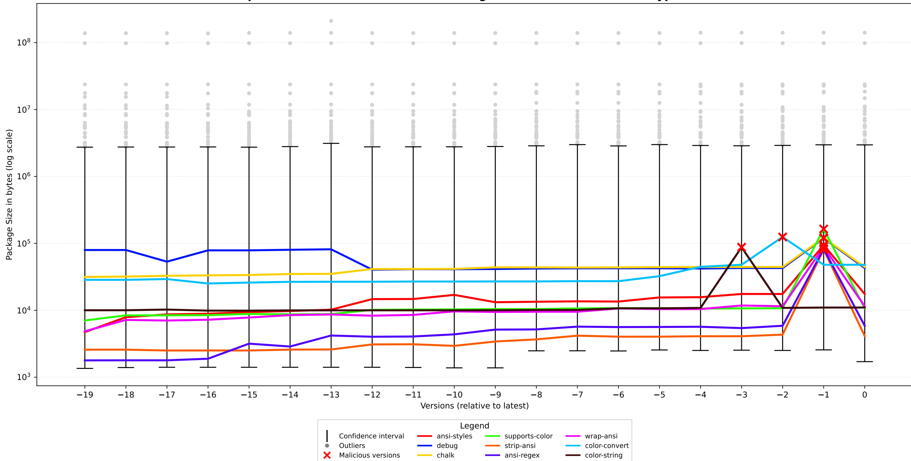
Comparison with Malware Dataset Package Size Metric - Attack B: Crypto attack
