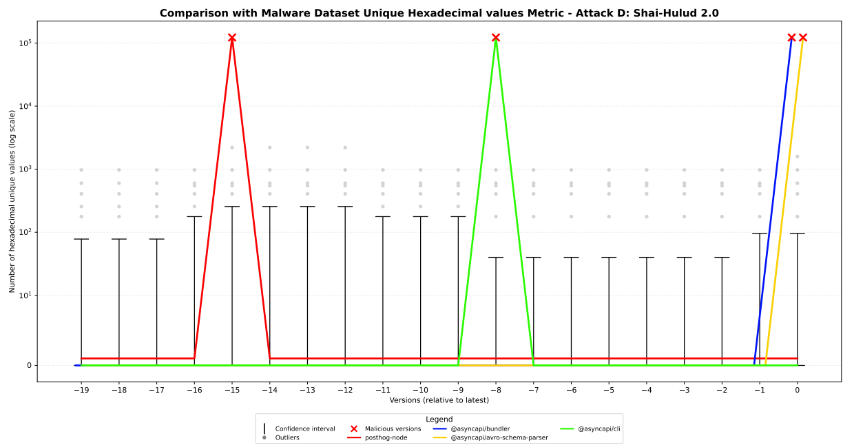
Figure 6.27: Comparison with Malware Dataset Unique Hexadecimal Values Metric for Attack D.
