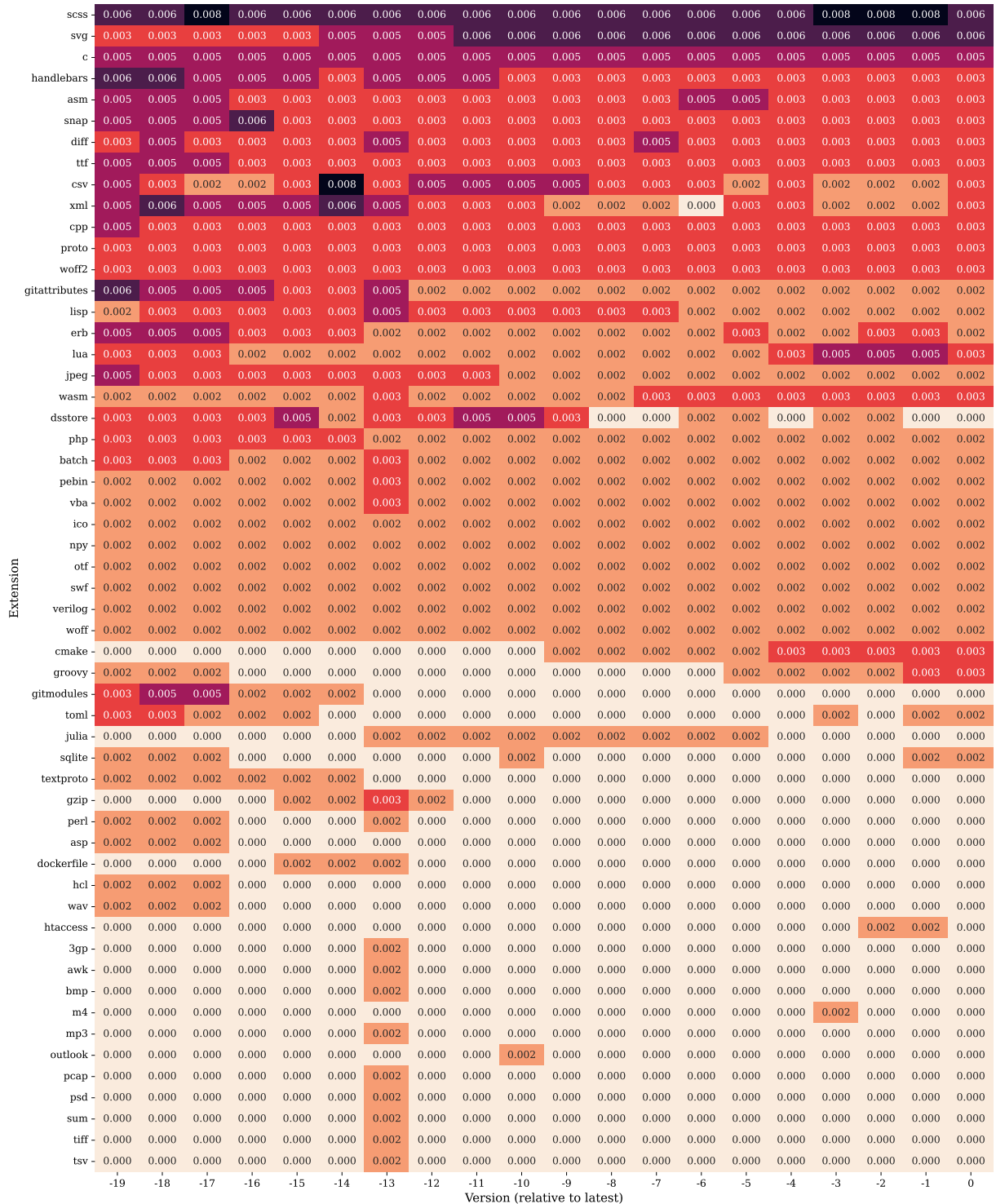
Figure 6.5: Heatmap for Rare File Types (Outliers).
