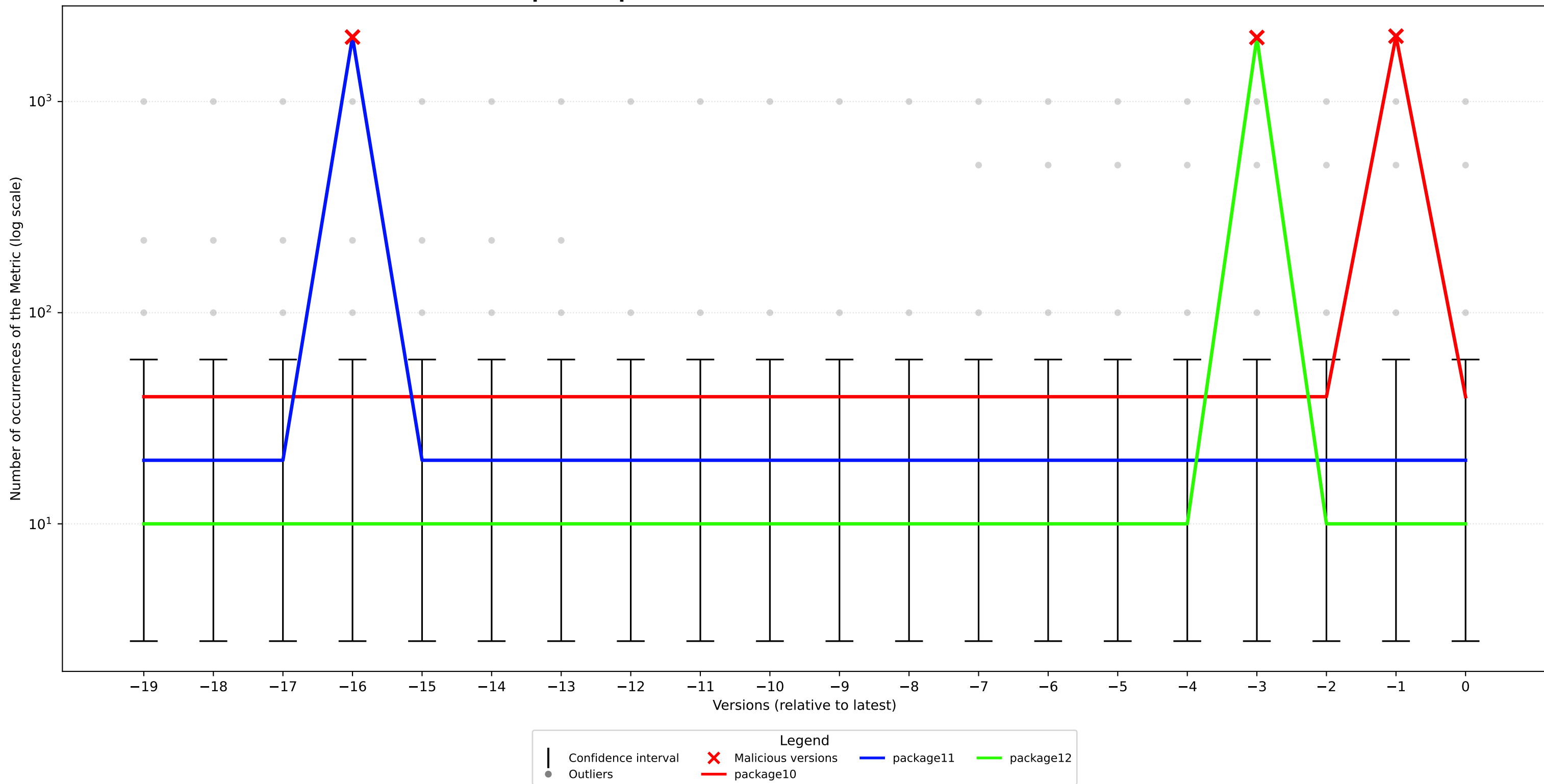
Example Comparison with Malware Metric - detectable attack
