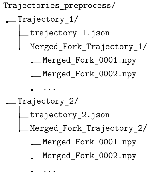
Figure 4.7 Directory structure of the preprocessed trajectory dataset.
