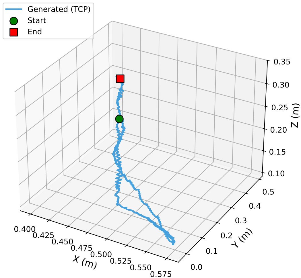
TCP Control Mode
