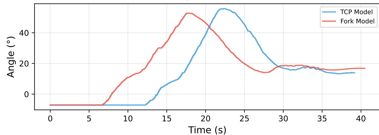
Joint 4 (Elbow)
