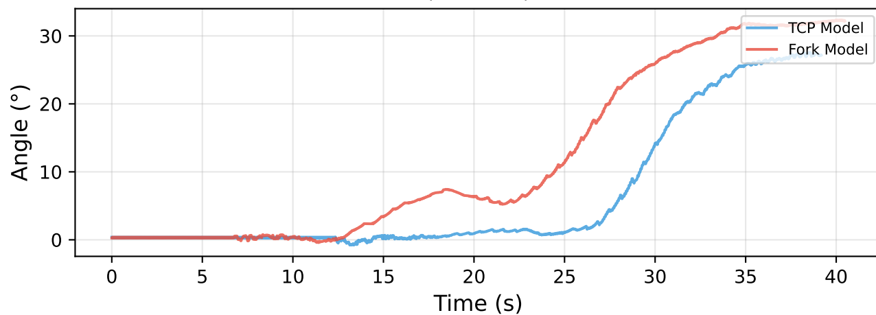
Joint 3 (Elbow)
