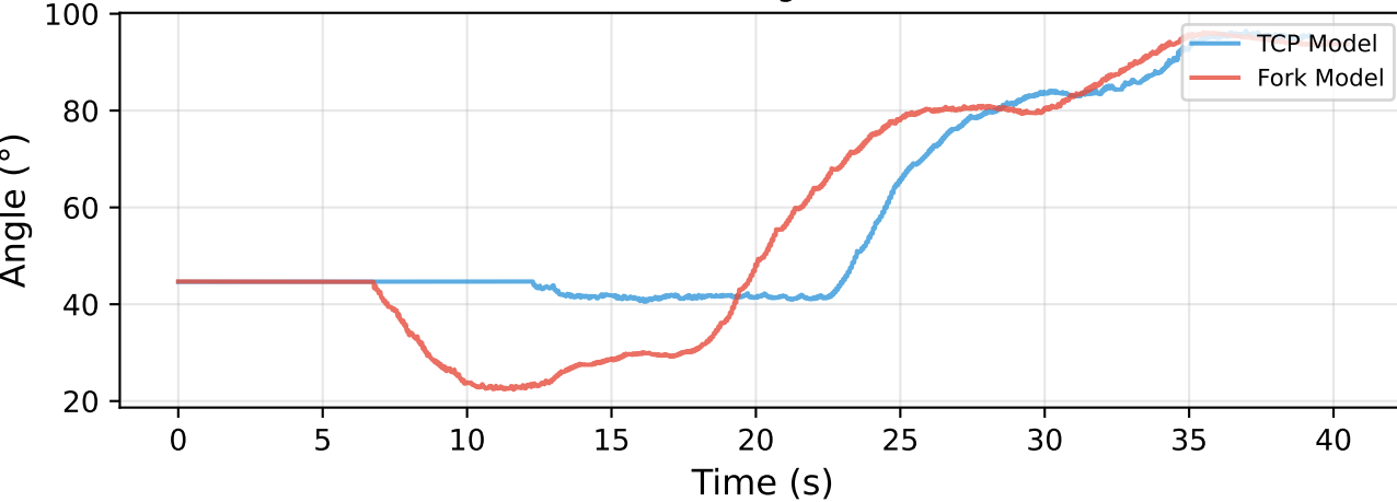
Joint 7 (Flange)
