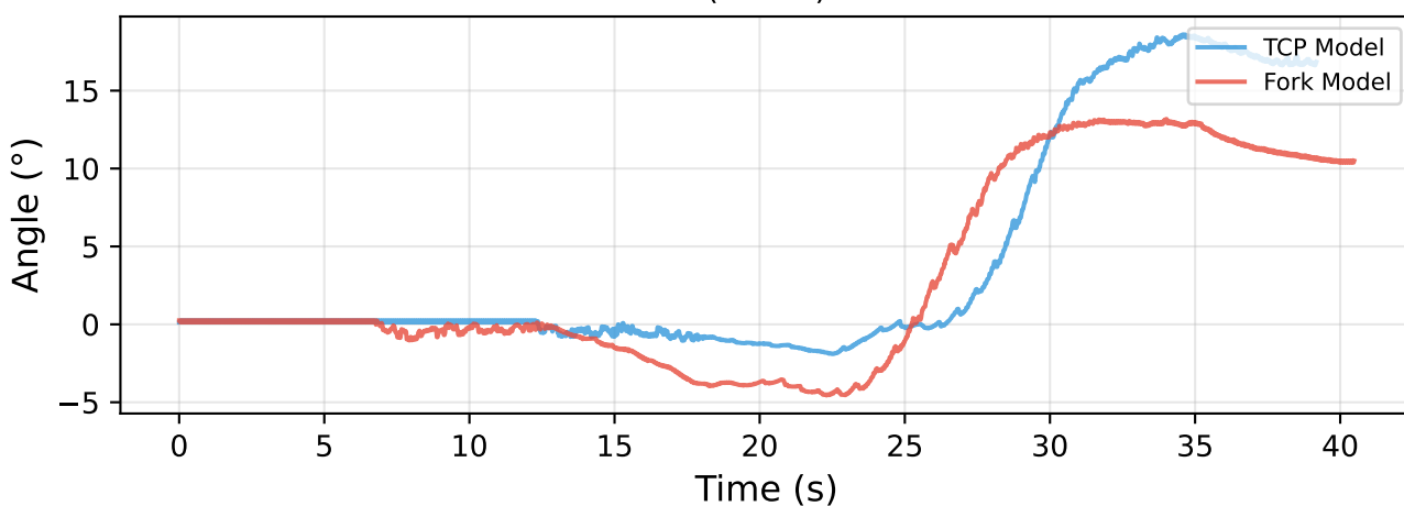
Joint 5 (Wrist)
