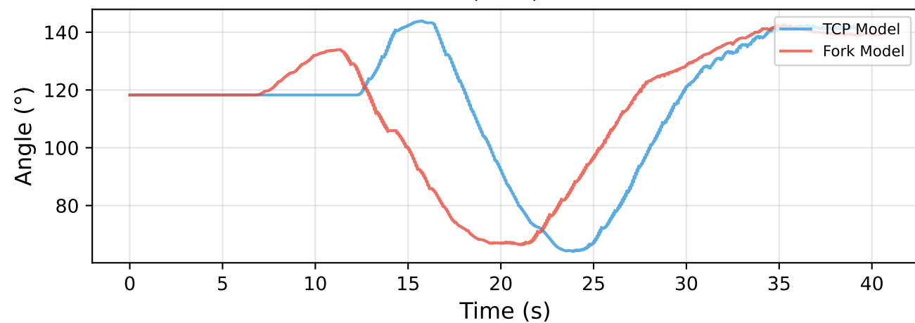
Joint 6 (Wrist)
