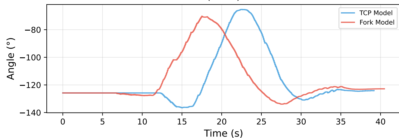
Joint 6 (Wrist)
