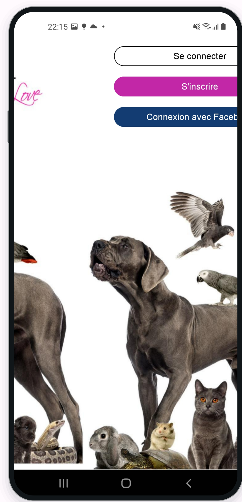
Authentication
