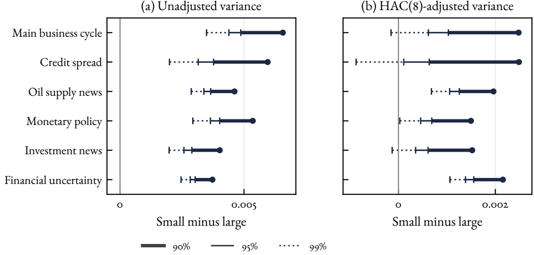
Figure D.1: Unadjusted and HAC(8)-Adjusted Coefficient Variance
