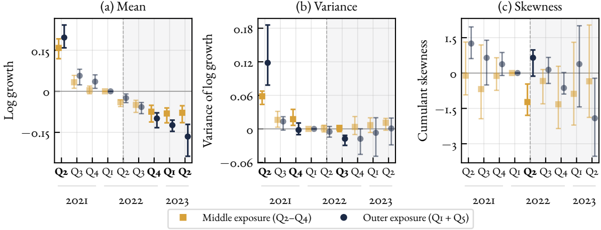
Figure C.5: Inflation Exposure and Growth-Distribution Changes
