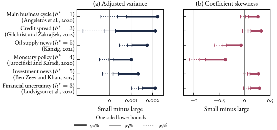
Figure 6: Shock-Mediated Distributional Responses by Firm Size
