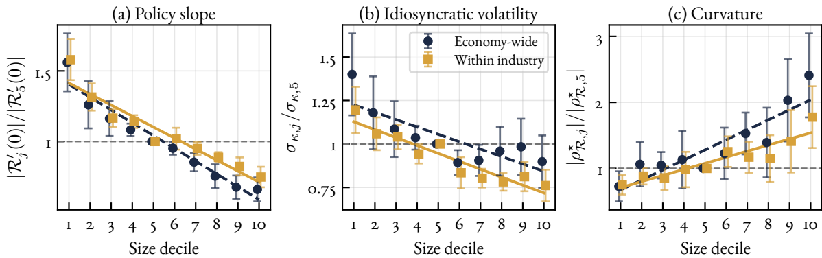
Figure E.1: Economy-Wide and Within-Industry Relative Policy Estimates
