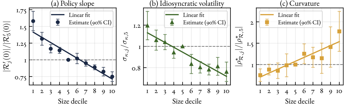
Figure 5: Relative Policy Slopes, Idiosyncratic Volatility, and Curvature Magnitude
