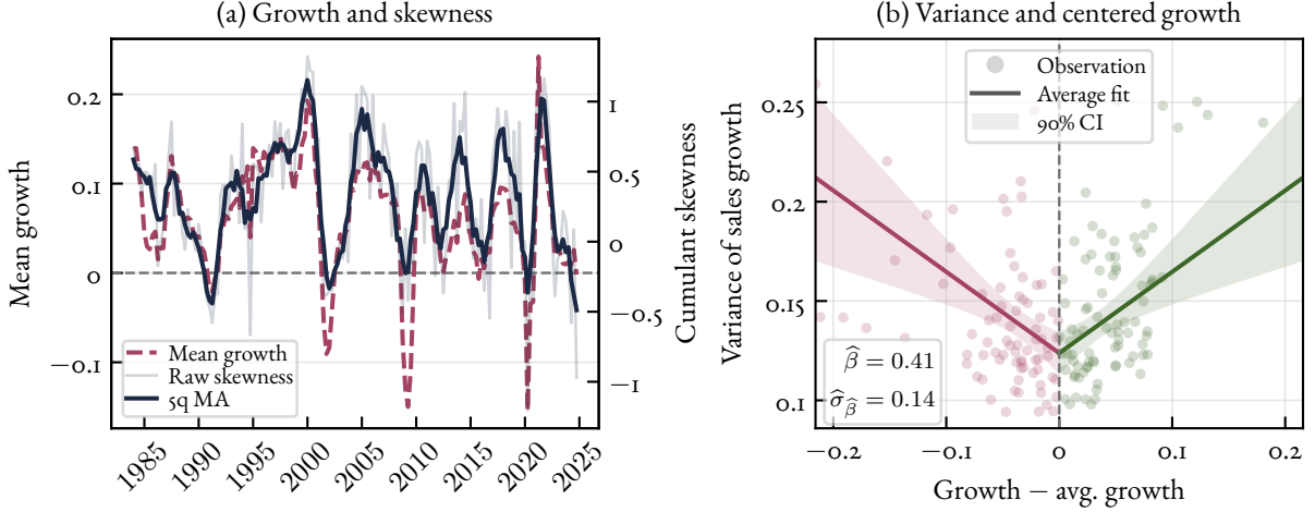
Figure 2: Growth, Cumulant Skewness, and Dispersion Around Trend
