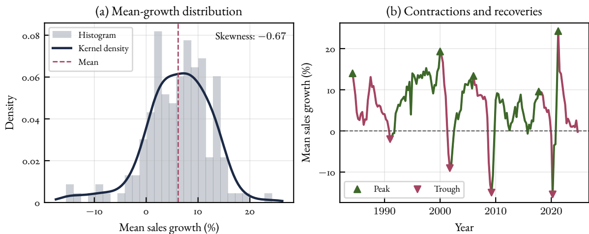
Figure C.1: Mean Growth Distribution and Turning Points
