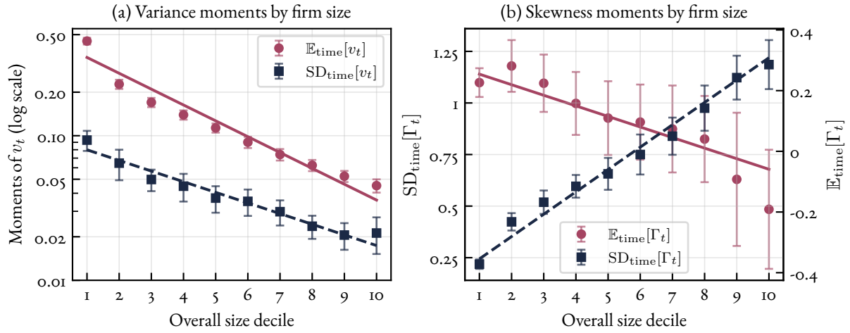
Figure C.2: Economy-Wide Opposing Size Gradients in Growth Moments
