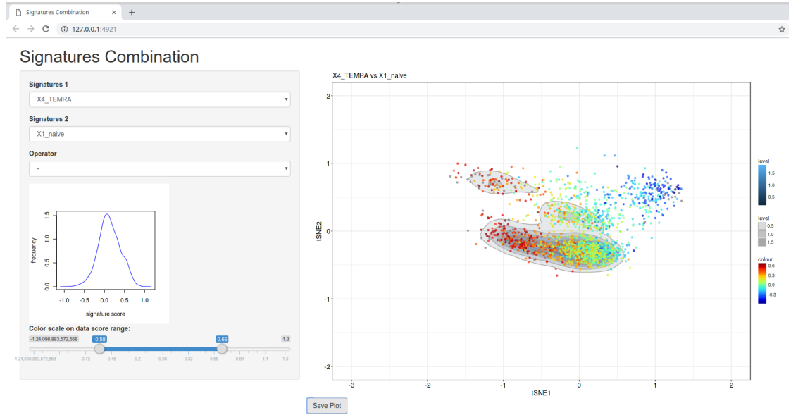
Figure 3: Screenshot of Single-Cell Signature Combiner. Signatures and operator can be selected with the drop-down menus on the left. The color scale of the map can be adjusted with the slider, according to the frequency histogram. The frequency of the combination scores is plotted against the signature score.
