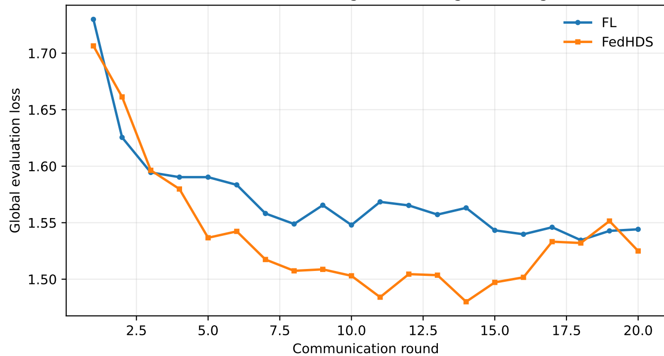
FL vs FedHDS convergence on Stage-2 setting
