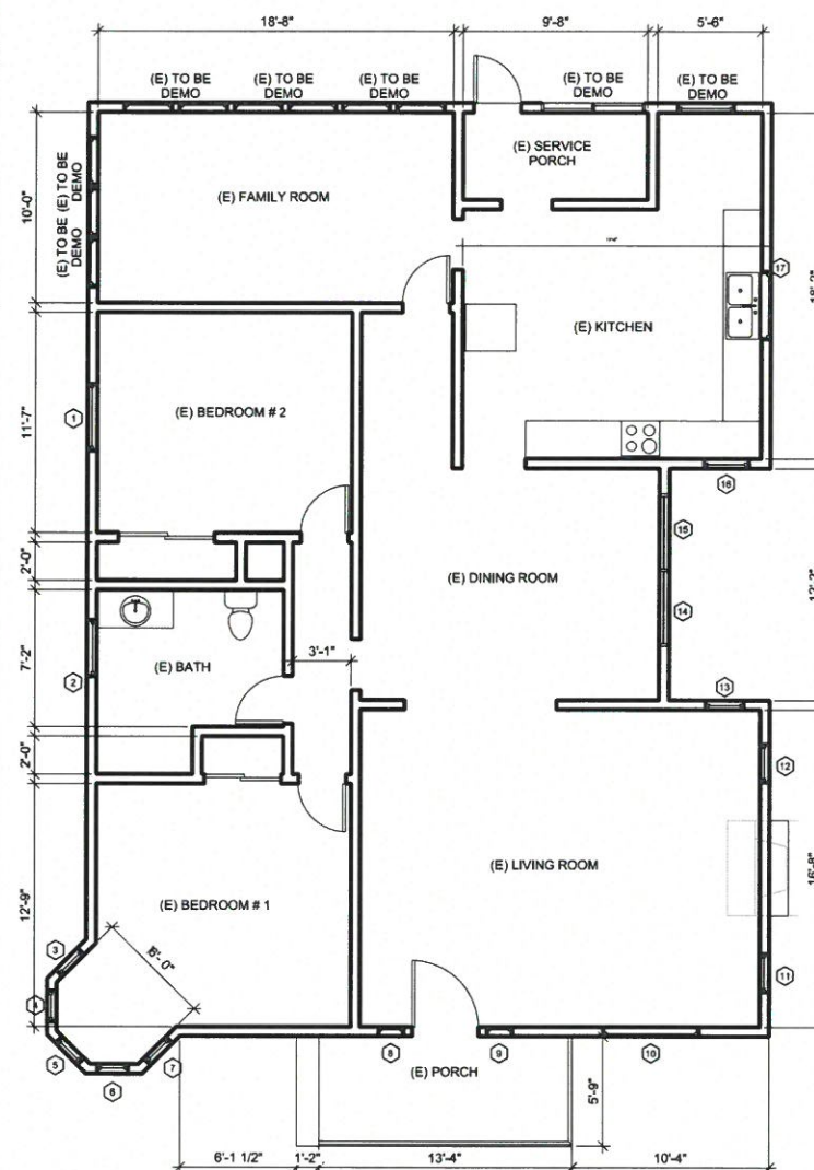
EXISTING PLAN
