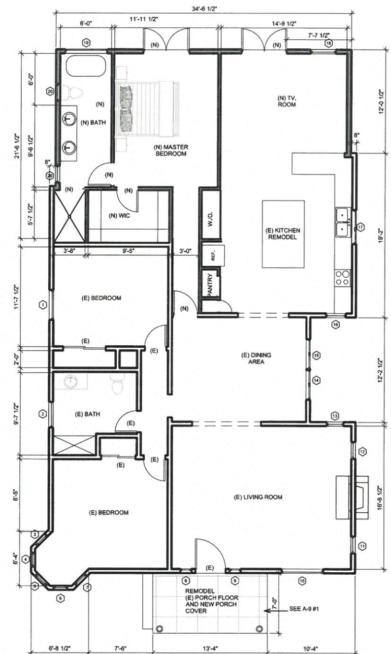
PROPOSED PLAN
