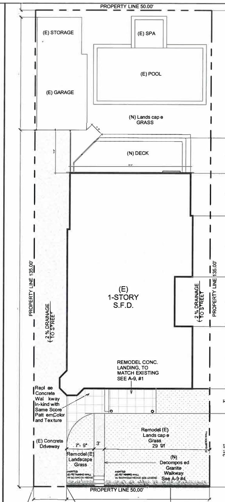
PROPOSED SITE AND LANDSCAPE PLAN
