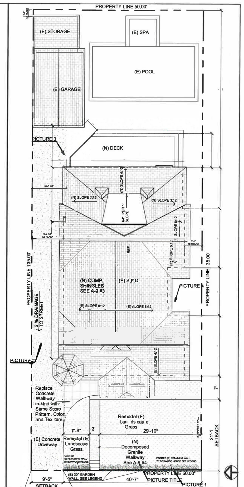
PROPOSED SITE AND ROOF PLAN
