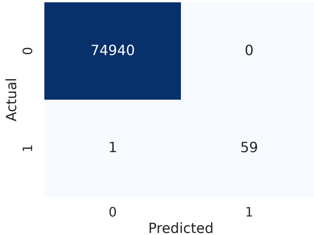
RQ2: Confusion Matrix - XGBoost (PS)
