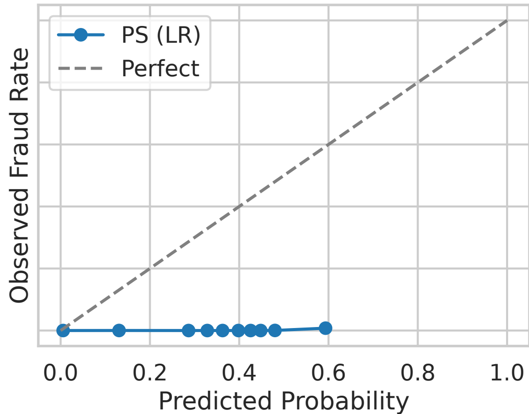
RQ3: Calibration - PS
