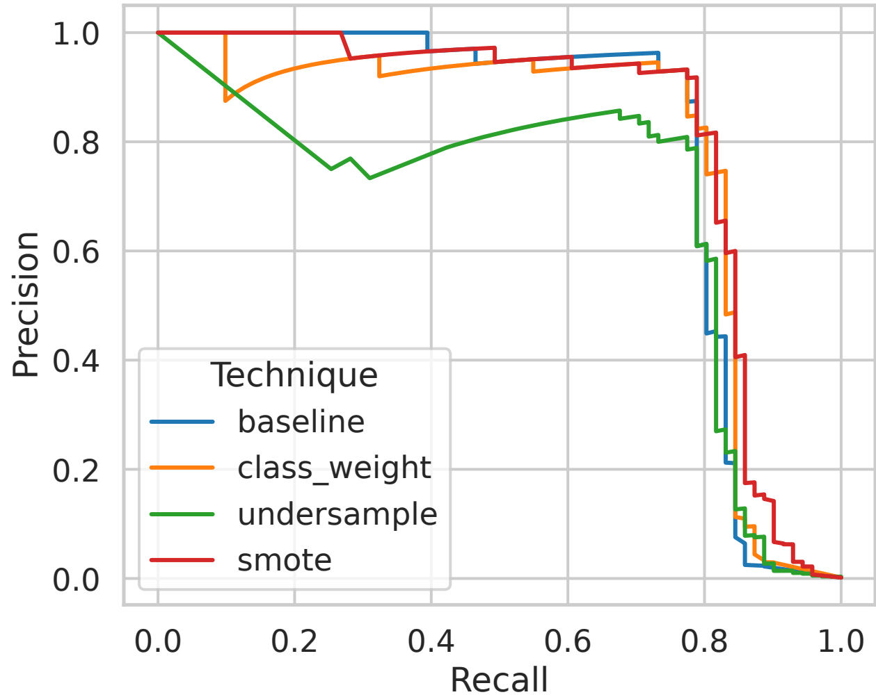
RQ1: PR Curves – RandomForest under different techniques (CC)
