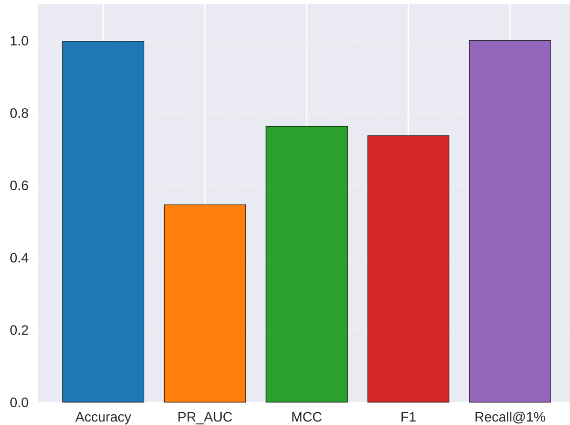
RQ4 — CreditCard: Metrics vs Accuracy
