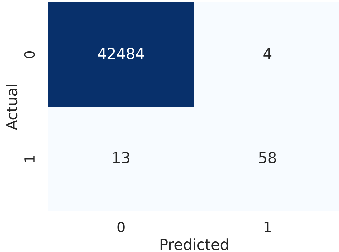
RQ2: Confusion Matrix - XGBoost (CC)
