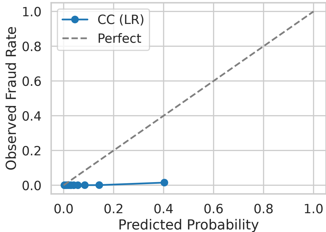
RQ3: Calibration - CC
