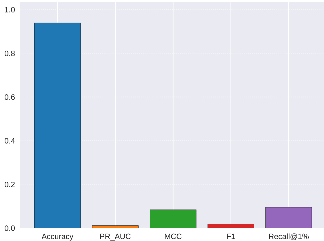
RQ4 — PaySim: Metrics vs Accuracy
