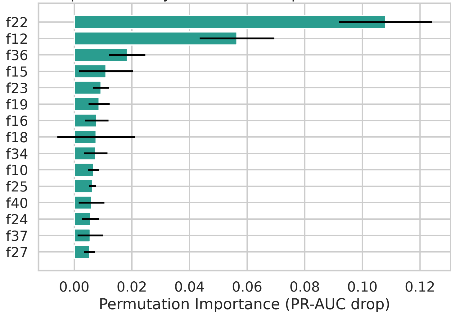
RQ2: Top Features by Permutation Importance - XGBoost (CC)
