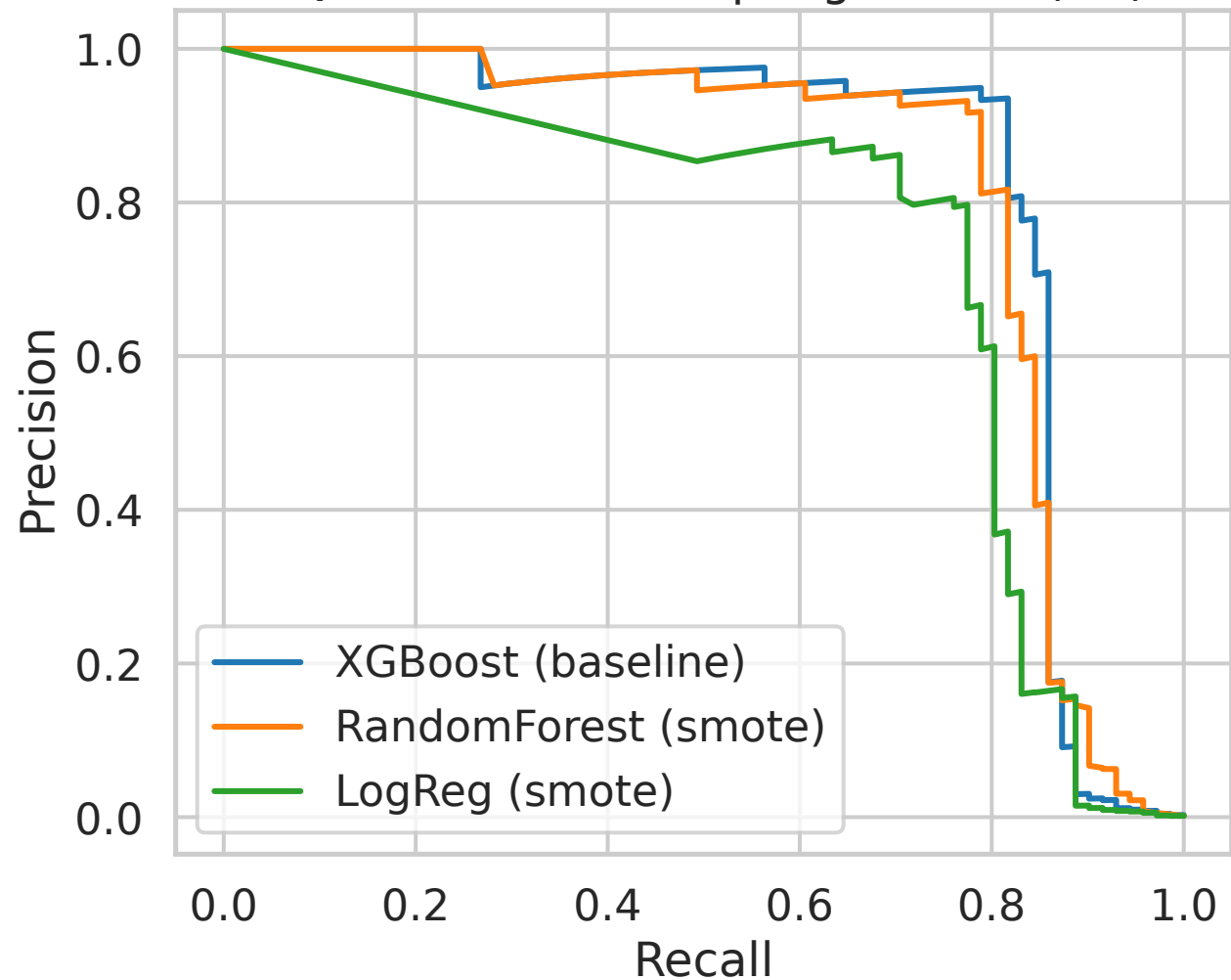
RQ2: PR Curves - Top Algorithms (CC)
