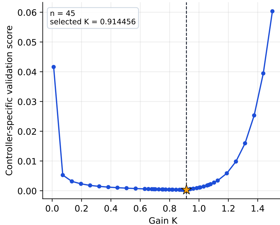
Global finite-time feedback
