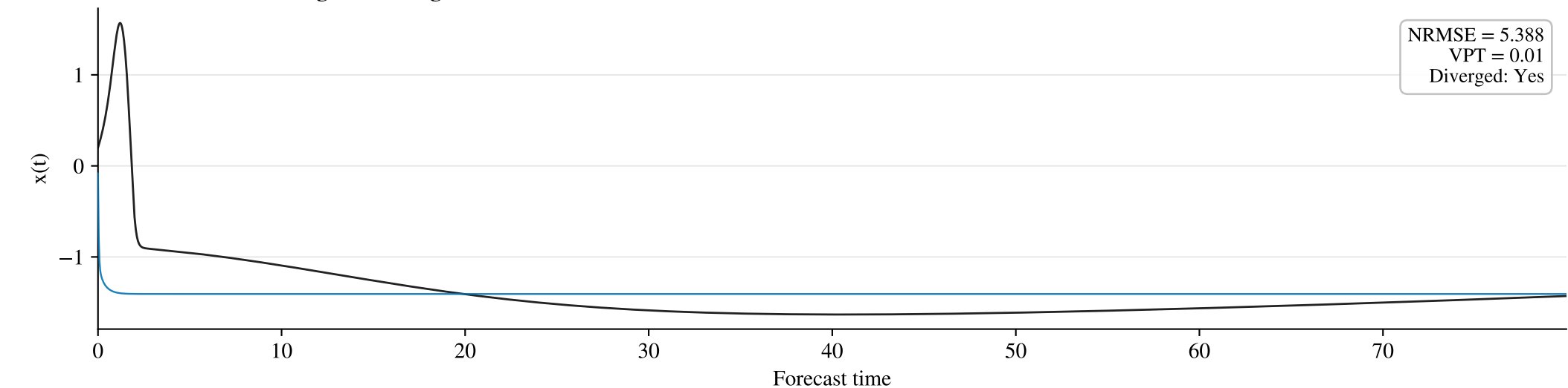
B CR: Chaotic \rightarrow Regular | target current I = 1.67
