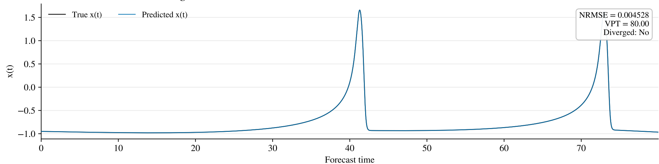
A CC: Chaotic \rightarrow Chaotic | target current I = 3.20
