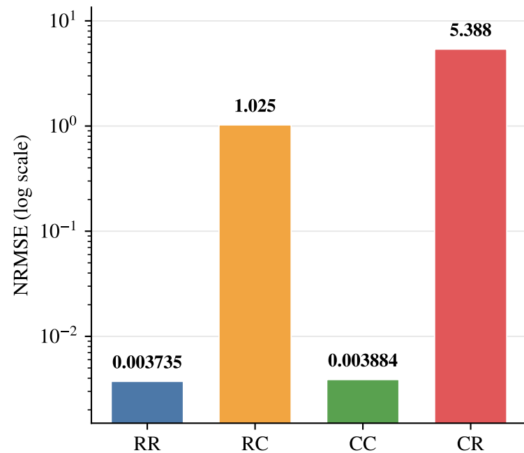
A Median NRMSE (log scale)
