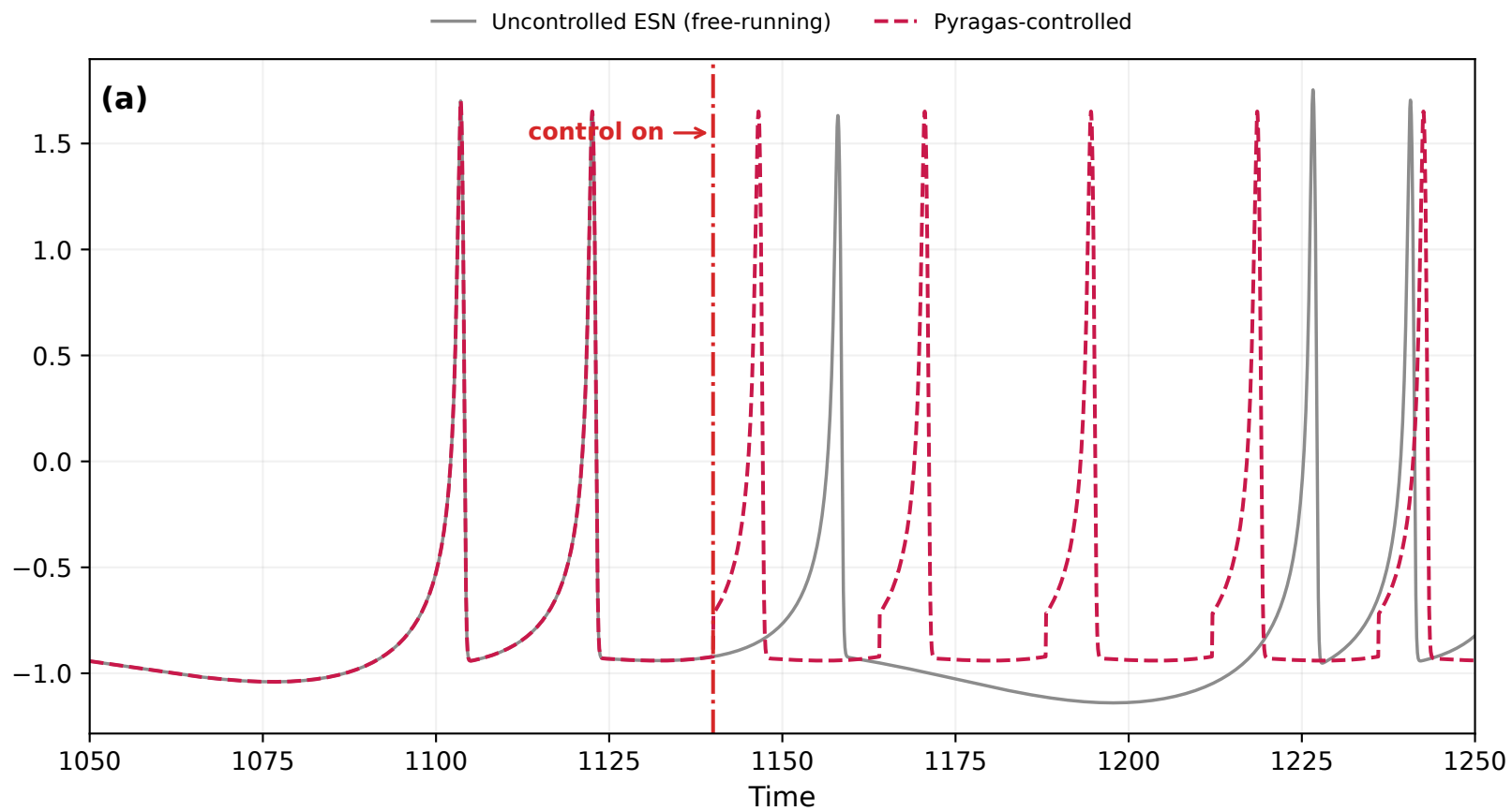
Hindmarsh-Rose x state
