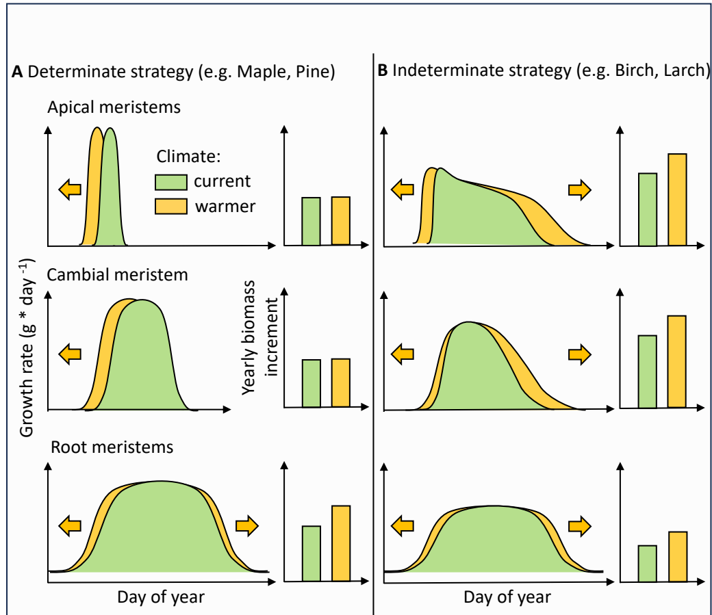
Figure 3: Hypothesized predictions of growth rates for the three major meristem (apical, cambium and root) classes of trees under current and warmer climates following an extreme determinate (A) and indeterminate (B) growth strategy. The area under the curve is summarized as yearly biomass increment in the respective bar-plot. Arrows indicate the shift of growth phenology under warmer climate conditions. Root meristems appear to be purely temperature opportunistic for both strategies, even growing during warm winter spells. The indicated genera were observed to showcase the illustrated trends. The responses of these two contrasting growth strategies might apply not only to different tree species but also within a population (e.g. along environmental gradients) and even within an individual as it transitions from the juvenile to the adult stage (ontogeny).
