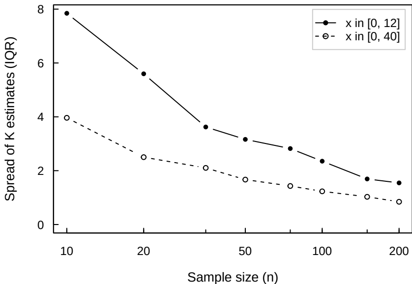
Range beats sample size
