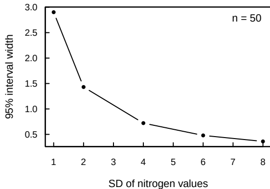
(c) Precision vs. spread of x
