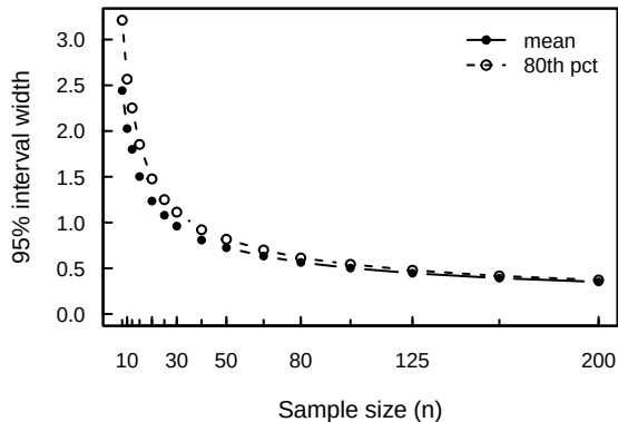
(a) Precision vs. sample size
