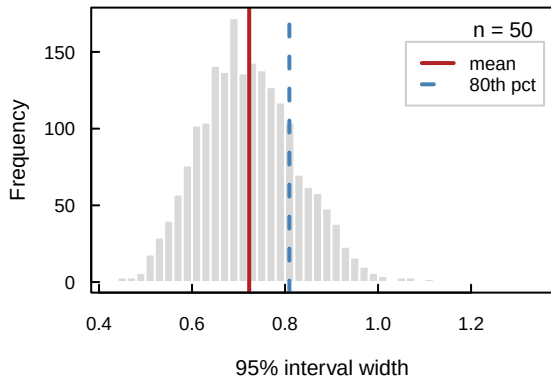
(b) Width varies between studies
