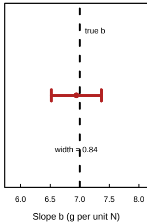
(c) Estimate and interval
