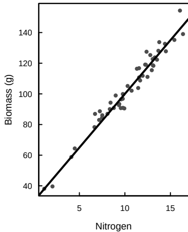
(a) Simulated data
