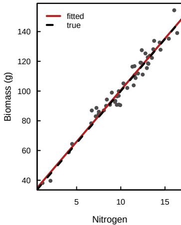
(b) Fitted and true line
