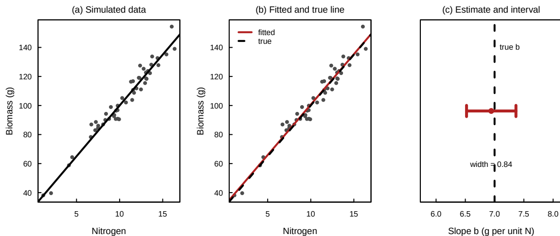
Figure 2: Step 2 of the loop for the linear example. (a) Data simulated from Equation 2 with a = 30 , b = 7 , \sigma = 5 and n = 50 : the hypothesis in visual form, showing effect size and scatter together. (b) The fitted model (solid) against the generating model (dashed), a check on the code rather than on the science. (c) The estimated slope and its 95% interval. The length of this bar is the quantity the rest of the section is about.
