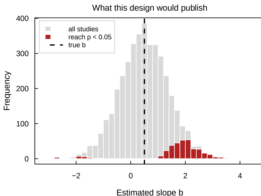
Figure 5: The distribution of slope estimates from 4000 simulated studies with b = 0.5 , \sigma = 15 and n = 20 (grey), and the subset that would reach p < 0.05 and so be most likely to be reported (dark). Conditional on significance, the design exaggerates the effect roughly fourfold and returns the wrong sign about 7% of the time. The dashed line is the true value.
