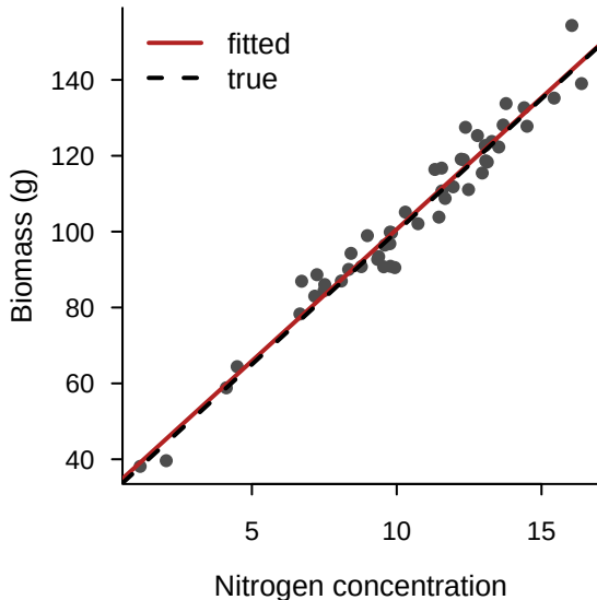
Fitted vs. generating model
