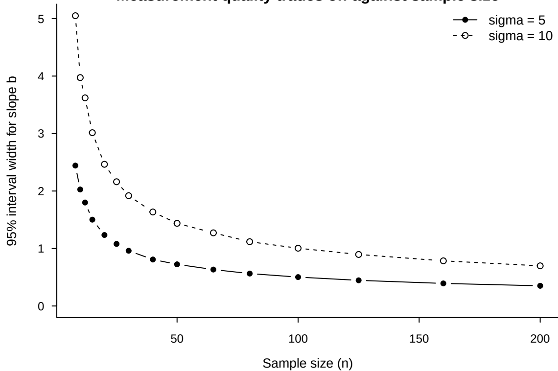
Measurement quality trades off against sample size
