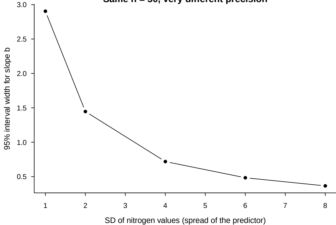
Same n = 50 , very different precision
